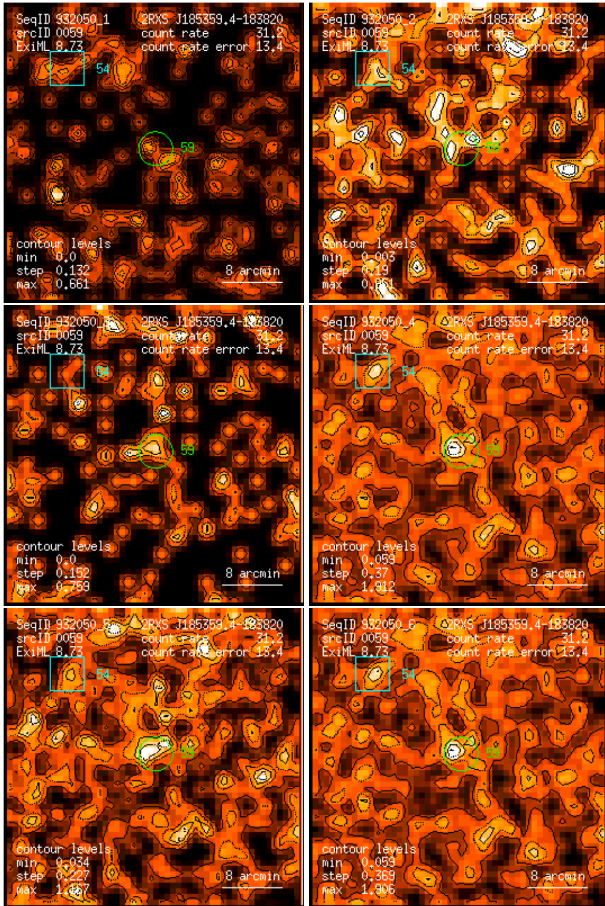
Figure 59: RASS 932050: detection 0059: band rate images, Gaussian filter: (1) PSPC channels 11 – 41, (2) 52 – 90, (3) 91 – 201, (4) 11 – 235, (5) 52 – 201, (6) 11 – 201. Broad band rates in counts/ks. Band rate contour levels in counts/ks/arcmin 2 .
