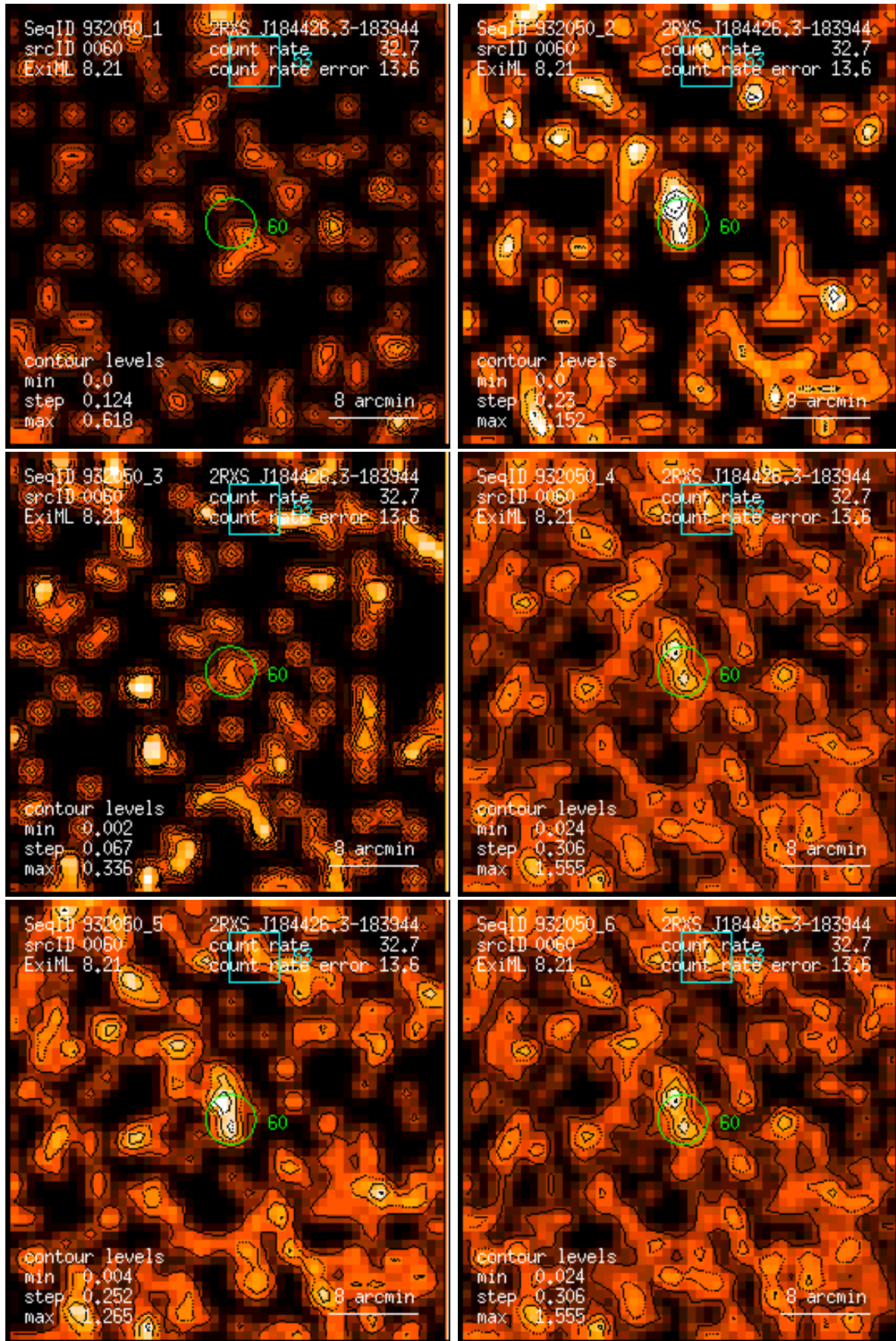
Figure 60: RASS 932050: detection 0060: band rate images, Gaussian filter: (1) PSPC channels 11 – 41, (2) 52 – 90, (3) 91 – 201, (4) 11 – 235, (5) 52 – 201, (6) 11 – 201. Broad band rates in counts/ks. Band rate contour levels in counts/ks/arcmin 2 .
