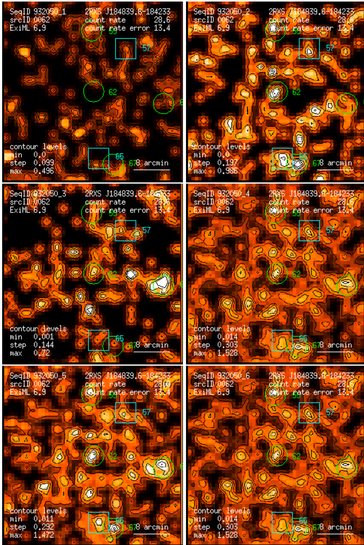
Figure 62: RASS 932050: detection 0062: band rate images, Gaussian filter: (1) PSPC channels 11 – 41, (2) 52 – 90, (3) 91 – 201, (4) 11 – 235, (5) 52 – 201, (6) 11 – 201. Broad band rates in counts/ks. Band rate contour levels in counts/ks/arcmin 2 .
