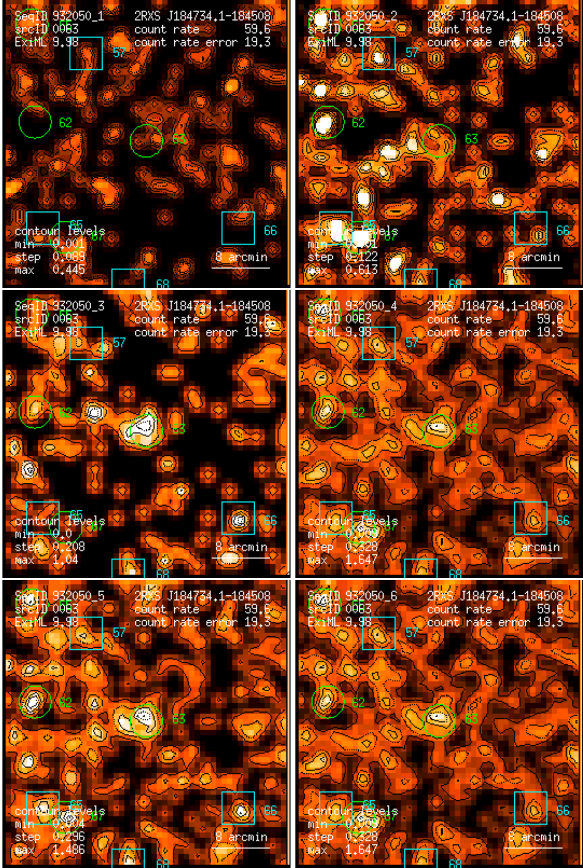
Figure 63: RASS 932050: detection 0063: band rate images, Gaussian filter: (1) PSPC channels 11 – 41, (2) 52 – 90, (3) 91 – 201, (4) 11 – 235, (5) 52 – 201, (6) 11 – 201. Broad band rates in counts/ks. Band rate contour levels in counts/ks/arcmin 2 .
