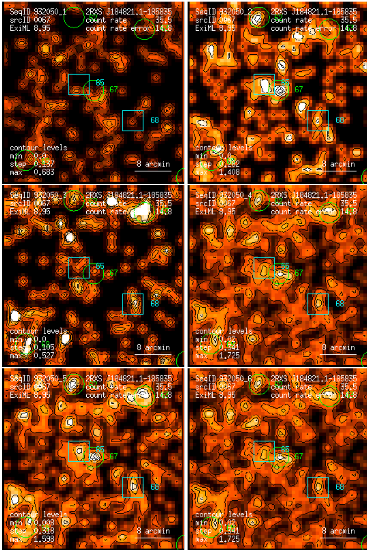
Figure 67: RASS 932050: detection 0067: band rate images, Gaussian filter: (1) PSPC channels 11 – 41, (2) 52 – 90, (3) 91 – 201, (4) 11 – 235, (5) 52 – 201, (6) 11 – 201. Broad band rates in counts/ks. Band rate contour levels in counts/ks/arcmin 2 .
