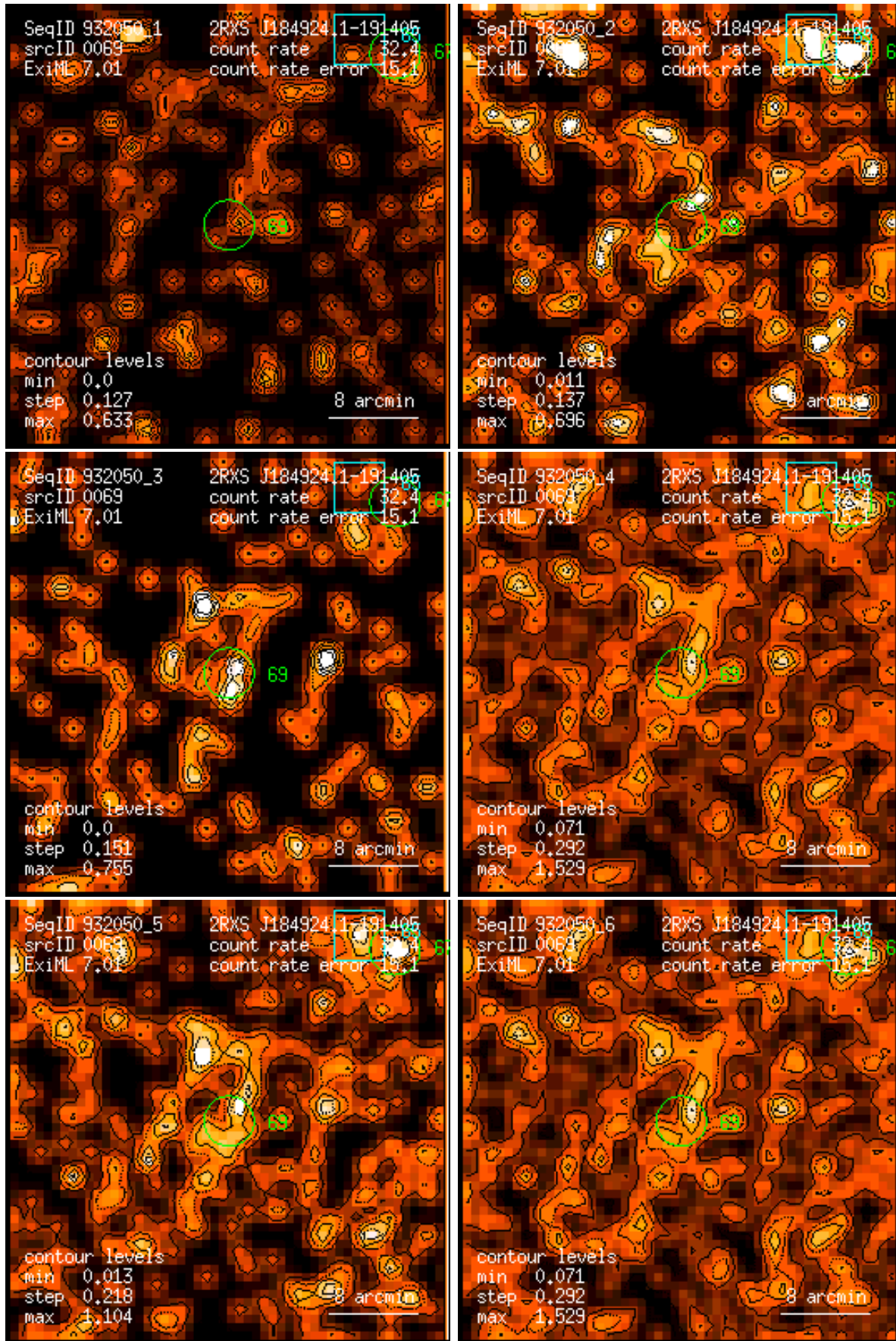
Figure 69: RASS 932050: detection 0069: band rate images, Gaussian filter: (1) PSPC channels 11 – 41, (2) 52 – 90, (3) 91 – 201, (4) 11 – 235, (5) 52 – 201, (6) 11 – 201. Broad band rates in counts/ks. Band rate contour levels in counts/ks/arcmin 2 .
