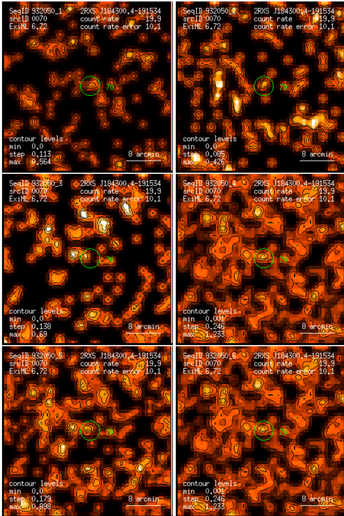
Figure 70: RASS 932050: detection 0070: band rate images, Gaussian filter: (1) PSPC channels 11 – 41, (2) 52 – 90, (3) 91 – 201, (4) 11 – 235, (5) 52 – 201, (6) 11 – 201. Broad band rates in counts/ks. Band rate contour levels in counts/ks/arcmin 2 .
