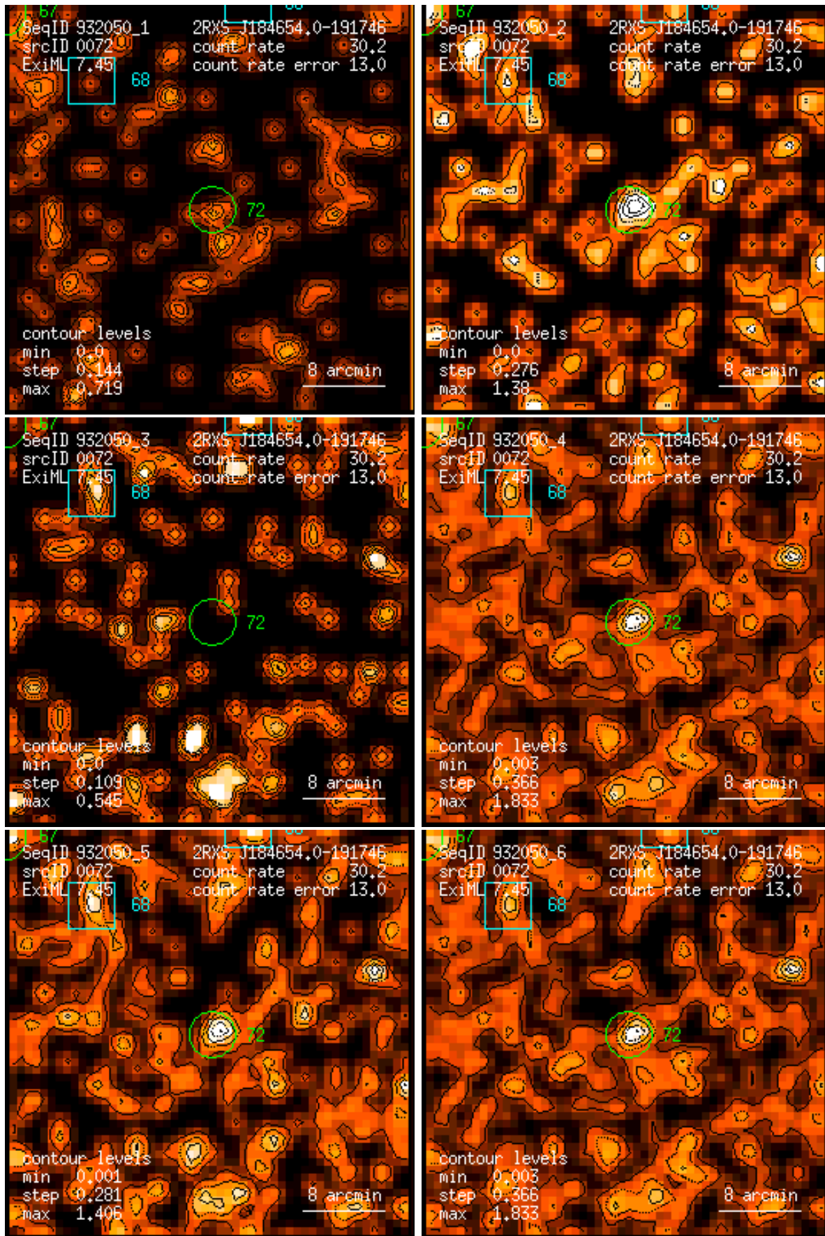
Figure 72: RASS 932050: detection 0072: band rate images, Gaussian filter: (1) PSPC channels 11 – 41, (2) 52 – 90, (3) 91 – 201, (4) 11 – 235, (5) 52 – 201, (6) 11 – 201. Broad band rates in counts/ks. Band rate contour levels in counts/ks/arcmin 2 .
