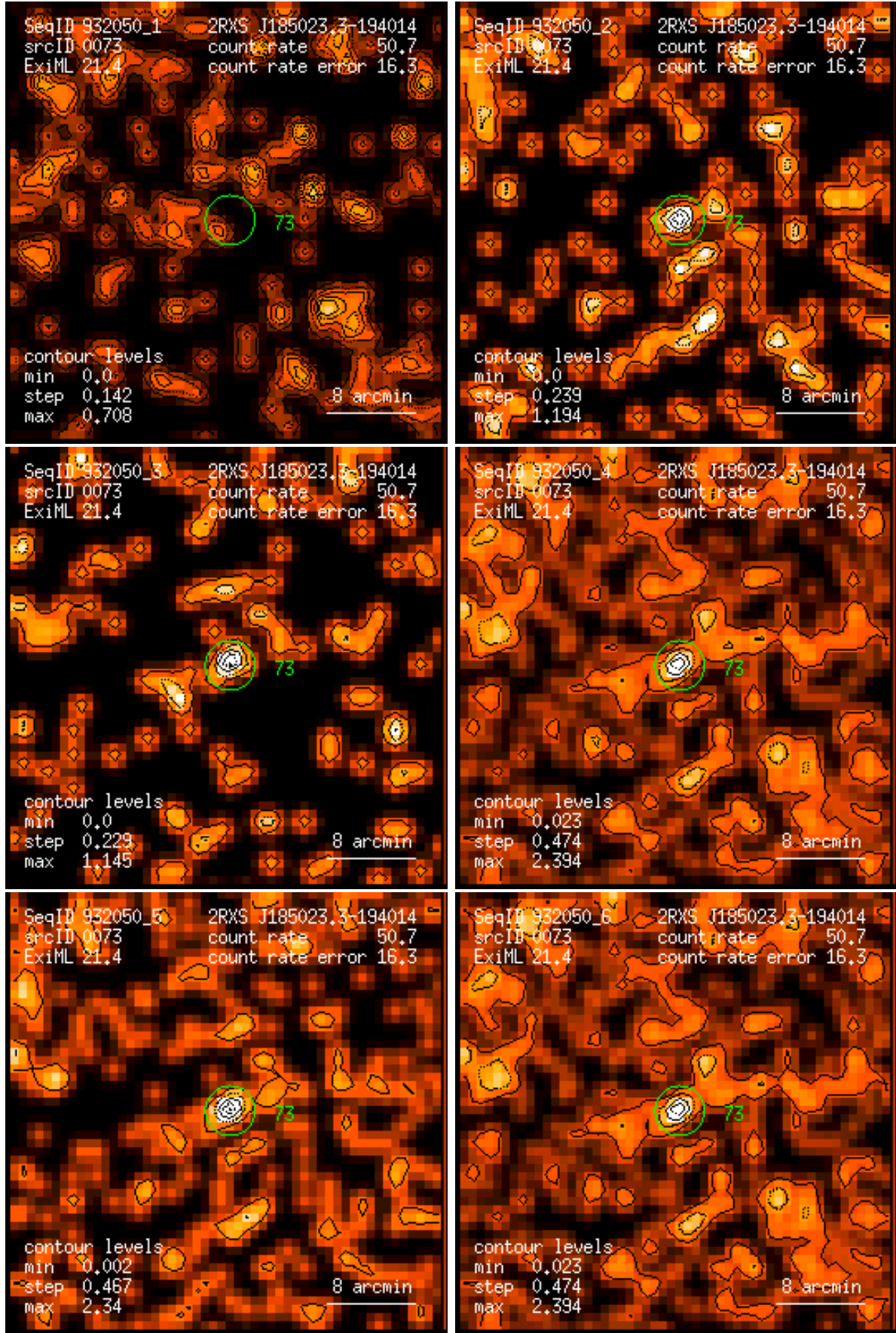
Figure 73: RASS 932050: detection 0073: band rate images, Gaussian filter: (1) PSPC channels 11 – 41, (2) 52 – 90, (3) 91 – 201, (4) 11 – 235, (5) 52 – 201, (6) 11 – 201. Broad band rates in counts/ks. Band rate contour levels in counts/ks/arcmin 2 .
