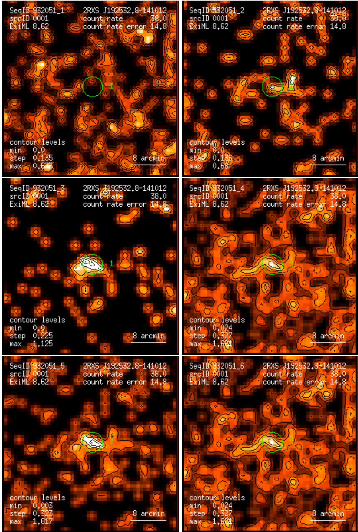
Figure 1: RASS 932051: detection 0001: band rate images, Gaussian filter: (1) PSPC channels 11 – 41, (2) 52 – 90, (3) 91 – 201, (4) 11 – 235, (5) 52 – 201, (6) 11 – 201. Broad band rates in counts/ks. Band rate contour levels in counts/ks/arcmin 2 .
