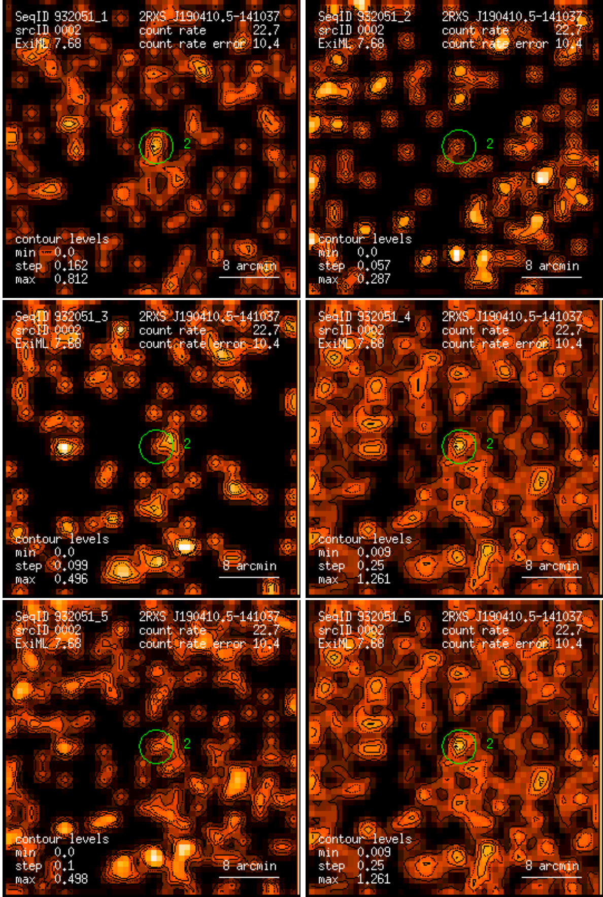
Figure 2: RASS 932051: detection 0002: band rate images, Gaussian filter: (1) PSPC channels 11 – 41, (2) 52 – 90, (3) 91 – 201, (4) 11 – 235, (5) 52 – 201, (6) 11 – 201. Broad band rates in counts/ks. Band rate contour levels in counts/ks/arcmin 2 .
