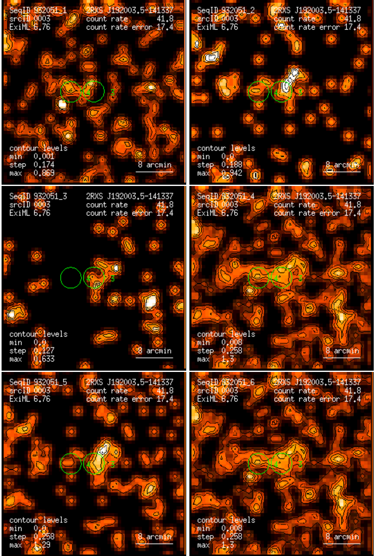
Figure 3: RASS 932051: detection 0003: band rate images, Gaussian filter: (1) PSPC channels 11 – 41, (2) 52 – 90, (3) 91 – 201, (4) 11 – 235, (5) 52 – 201, (6) 11 – 201. Broad band rates in counts/ks. Band rate contour levels in counts/ks/arcmin 2 .
