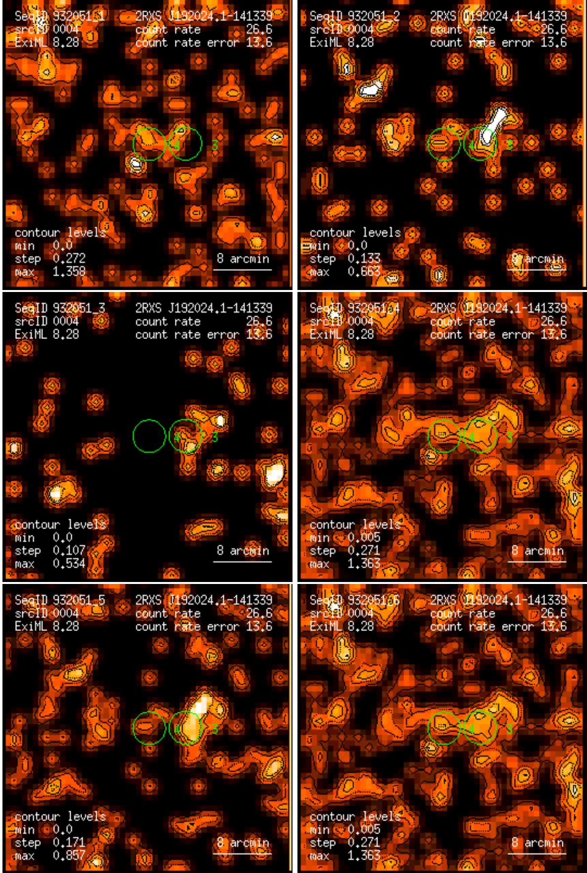
Figure 4: RASS 932051: detection 0004: band rate images, Gaussian filter: (1) PSPC channels 11 – 41, (2) 52 – 90, (3) 91 – 201, (4) 11 – 235, (5) 52 – 201, (6) 11 – 201. Broad band rates in counts/ks. Band rate contour levels in counts/ks/arcmin 2 .
