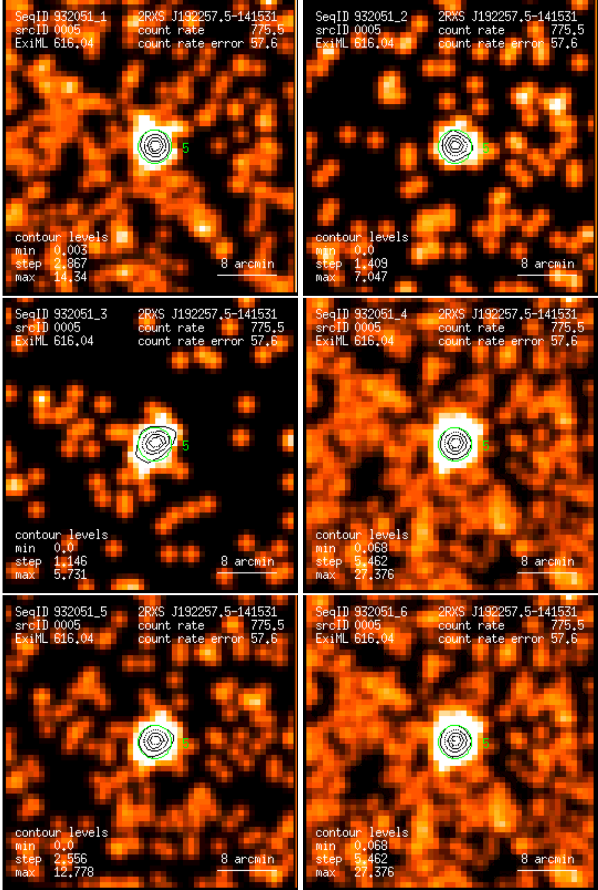
Figure 5: RASS 932051: detection 0005: band rate images, Gaussian filter: (1) PSPC channels 11 – 41, (2) 52 – 90, (3) 91 – 201, (4) 11 – 235, (5) 52 – 201, (6) 11 – 201. Broad band rates in counts/ks. Band rate contour levels in counts/ks/arcmin 2 .
