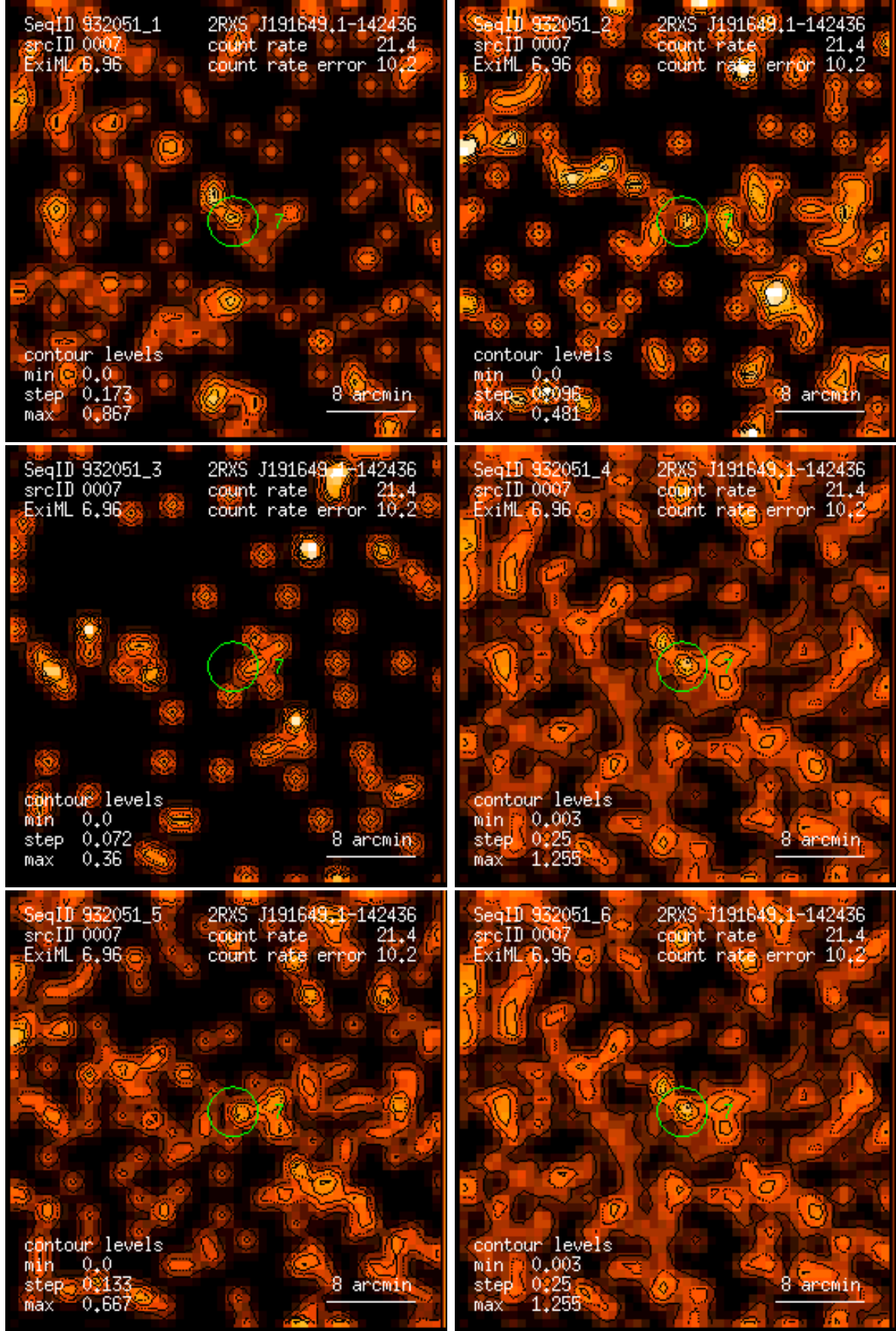
Figure 7: RASS 932051: detection 0007: band rate images, Gaussian filter: (1) PSPC channels 11 – 41, (2) 52 – 90, (3) 91 – 201, (4) 11 – 235, (5) 52 – 201, (6) 11 – 201. Broad band rates in counts/ks. Band rate contour levels in counts/ks/arcmin 2 .
