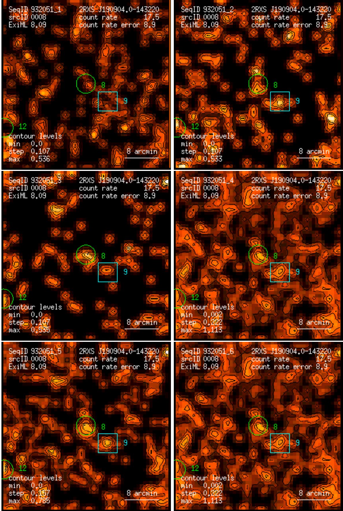
Figure 8: RASS 932051: detection 0008: band rate images, Gaussian filter: (1) PSPC channels 11 – 41, (2) 52 – 90, (3) 91 – 201, (4) 11 – 235, (5) 52 – 201, (6) 11 – 201. Broad band rates in counts/ks. Band rate contour levels in counts/ks/arcmin 2 .
