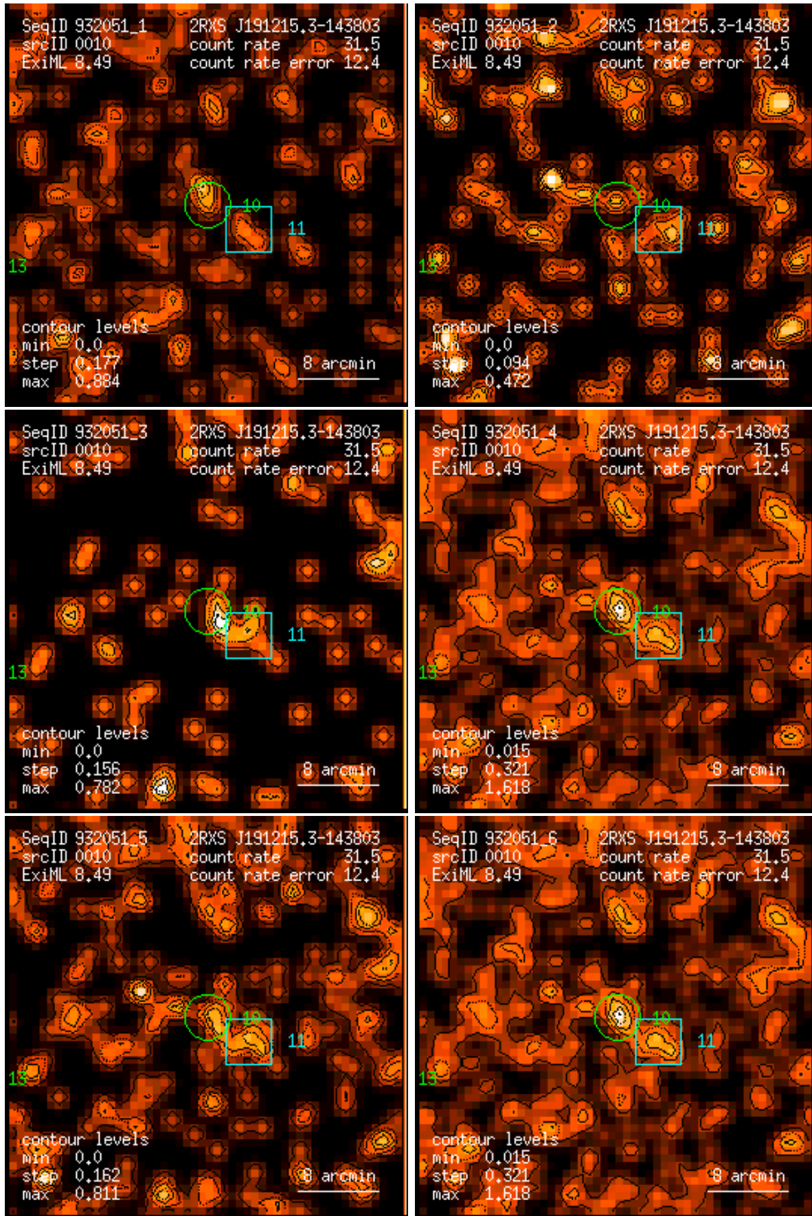
Figure 10: RASS 932051: detection 0010: band rate images, Gaussian filter: (1) PSPC channels 11 – 41, (2) 52 – 90, (3) 91 – 201, (4) 11 – 235, (5) 52 – 201, (6) 11 – 201. Broad band rates in counts/ks. Band rate contour levels in counts/ks/arcmin 2 .
