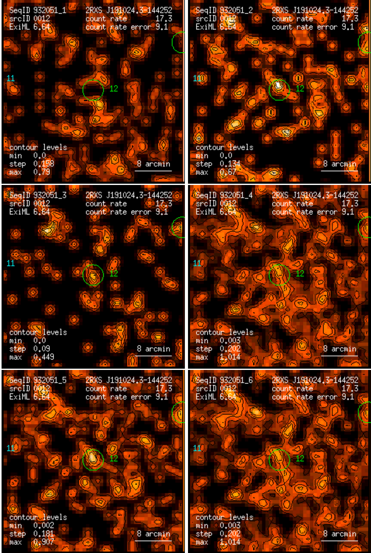
Figure 12: RASS 932051: detection 0012: band rate images, Gaussian filter: (1) PSPC channels 11 – 41, (2) 52 – 90, (3) 91 – 201, (4) 11 – 235, (5) 52 – 201, (6) 11 – 201. Broad band rates in counts/ks. Band rate contour levels in counts/ks/arcmin 2 .
