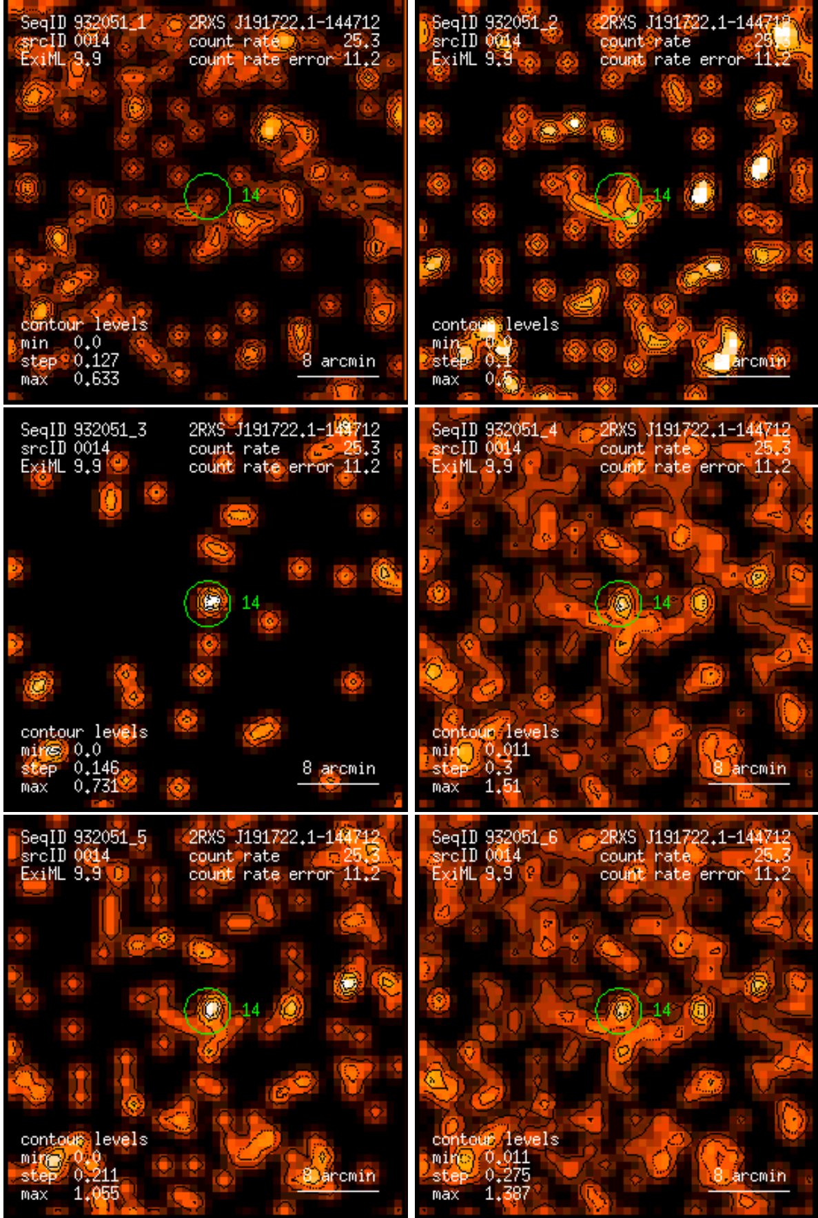
Figure 14: RASS 932051: detection 0014: band rate images, Gaussian filter: (1) PSPC channels 11 – 41, (2) 52 – 90, (3) 91 – 201, (4) 11 – 235, (5) 52 – 201, (6) 11 – 201. Broad band rates in counts/ks. Band rate contour levels in counts/ks/arcmin 2 .
