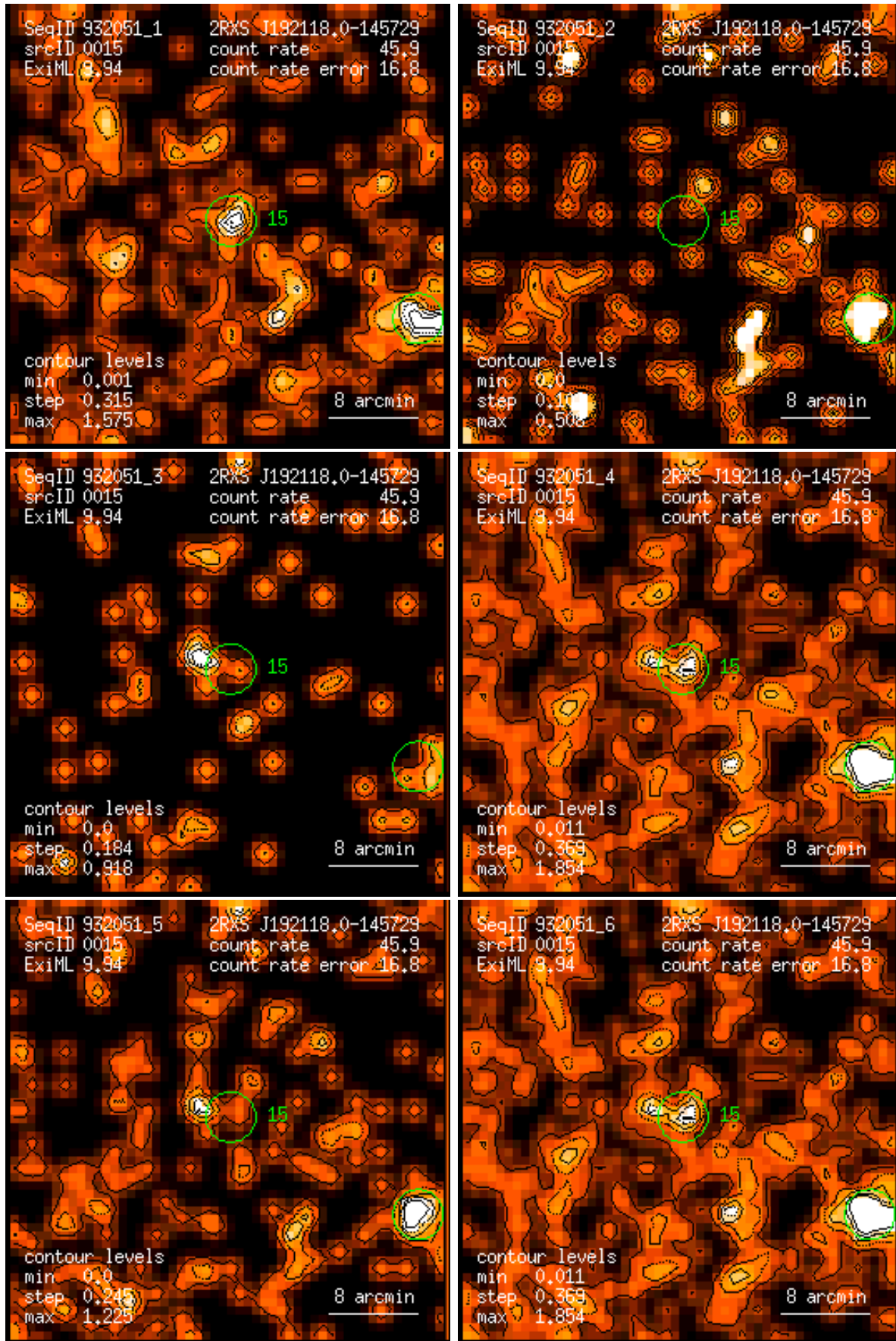
Figure 15: RASS 932051: detection 0015: band rate images, Gaussian filter: (1) PSPC channels 11 – 41, (2) 52 – 90, (3) 91 – 201, (4) 11 – 235, (5) 52 – 201, (6) 11 – 201. Broad band rates in counts/ks. Band rate contour levels in counts/ks/arcmin 2 .
