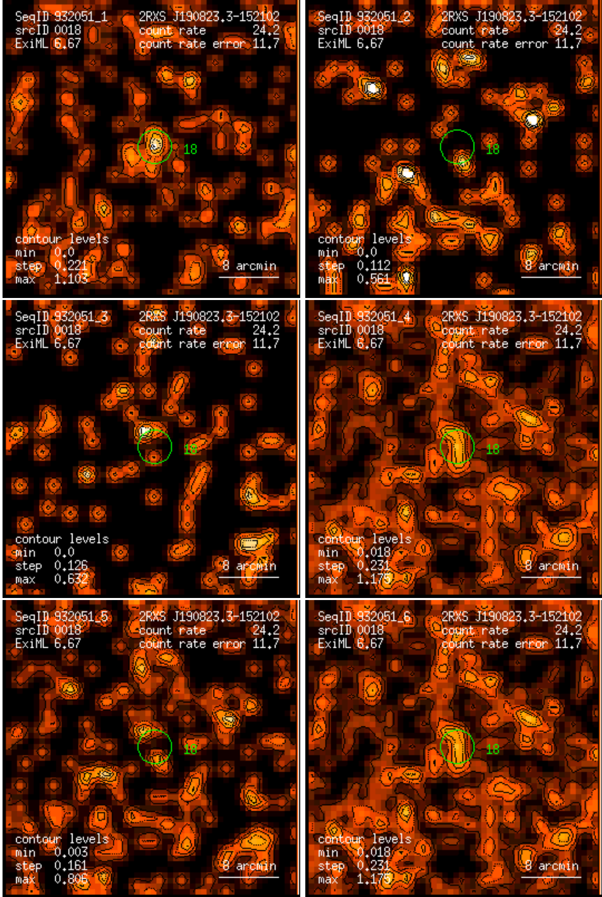
Figure 18: RASS 932051: detection 0018: band rate images, Gaussian filter: (1) PSPC channels 11 – 41, (2) 52 – 90, (3) 91 – 201, (4) 11 – 235, (5) 52 – 201, (6) 11 – 201. Broad band rates in counts/ks. Band rate contour levels in counts/ks/arcmin 2 .
