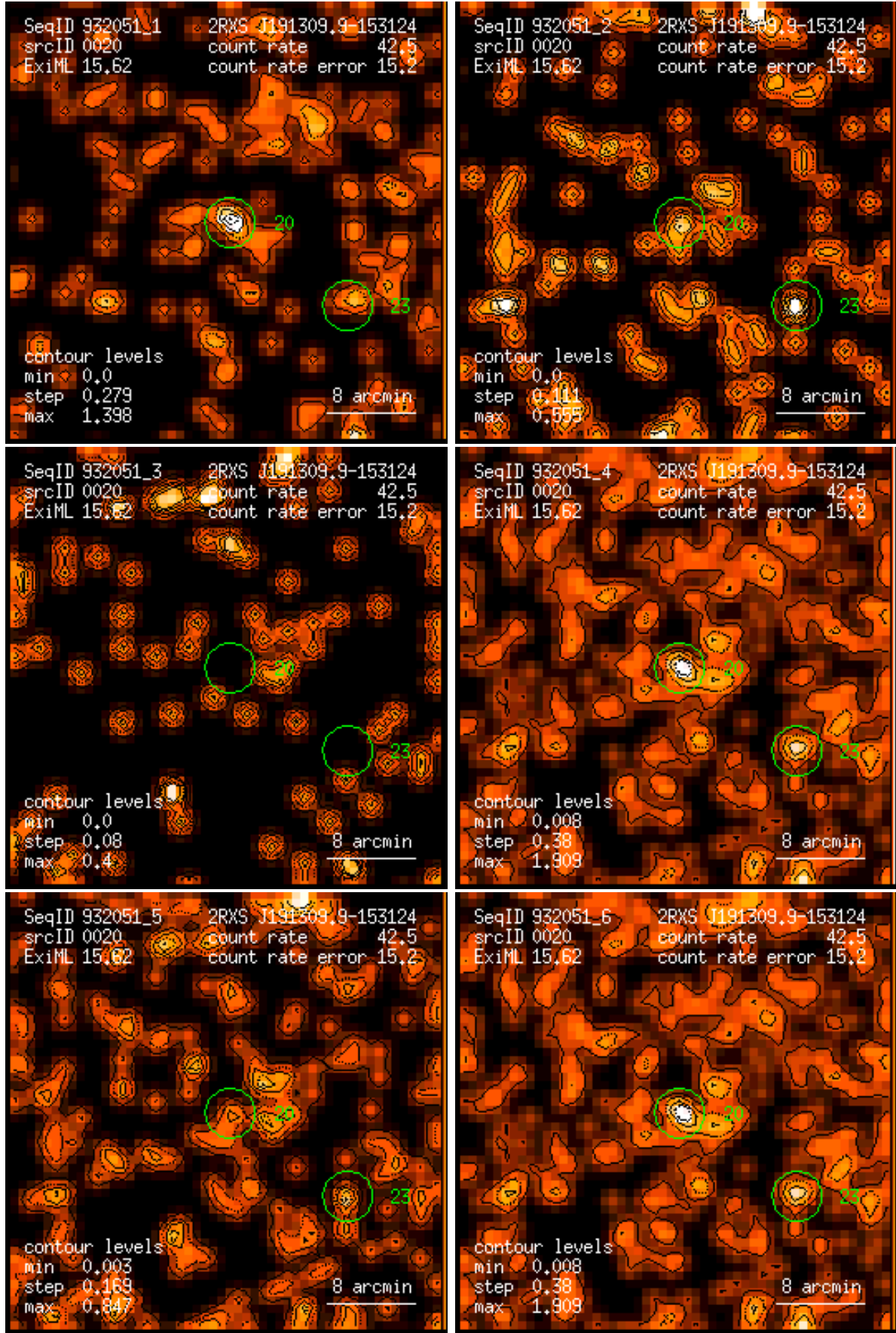
Figure 20: RASS 932051: detection 0020: band rate images, Gaussian filter: (1) PSPC channels 11 – 41, (2) 52 – 90, (3) 91 – 201, (4) 11 – 235, (5) 52 – 201, (6) 11 – 201. Broad band rates in counts/ks. Band rate contour levels in counts/ks/arcmin 2 .
