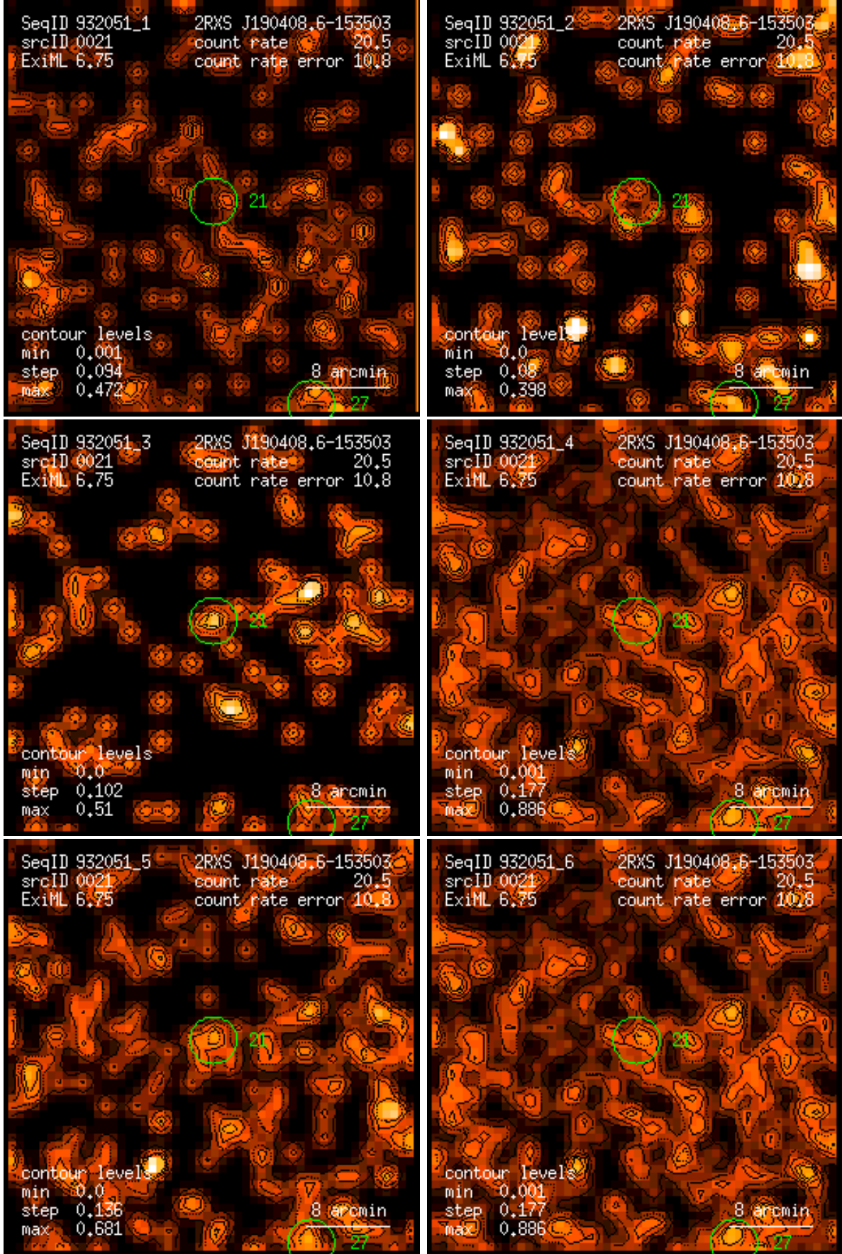
Figure 21: RASS 932051: detection 0021: band rate images, Gaussian filter: (1) PSPC channels 11 – 41, (2) 52 – 90, (3) 91 – 201, (4) 11 – 235, (5) 52 – 201, (6) 11 – 201. Broad band rates in counts/ks. Band rate contour levels in counts/ks/arcmin 2 .
