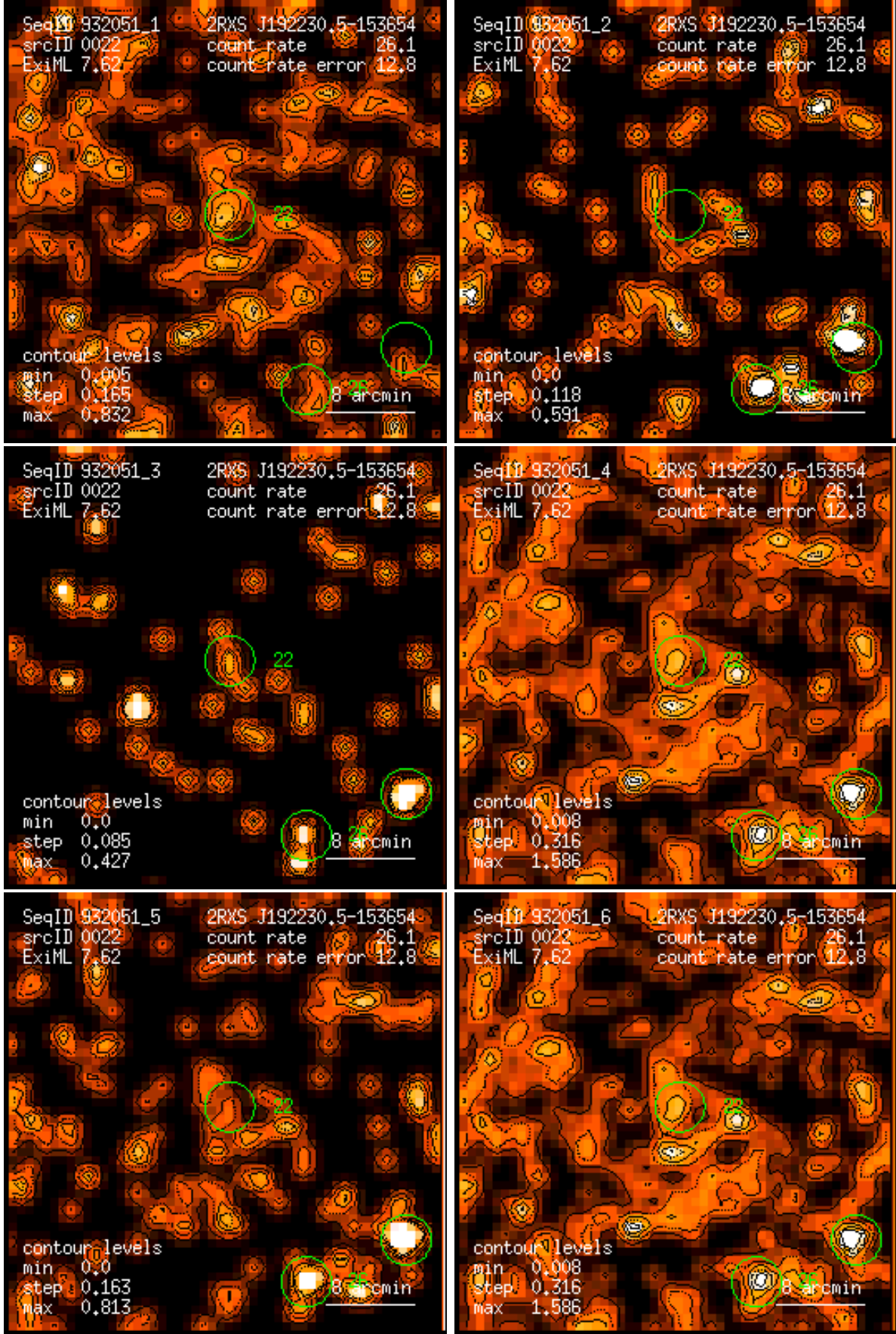
Figure 22: RASS 932051: detection 0022: band rate images, Gaussian filter: (1) PSPC channels 11 – 41, (2) 52 – 90, (3) 91 – 201, (4) 11 – 235, (5) 52 – 201, (6) 11 – 201. Broad band rates in counts/ks. Band rate contour levels in counts/ks/arcmin 2 .
