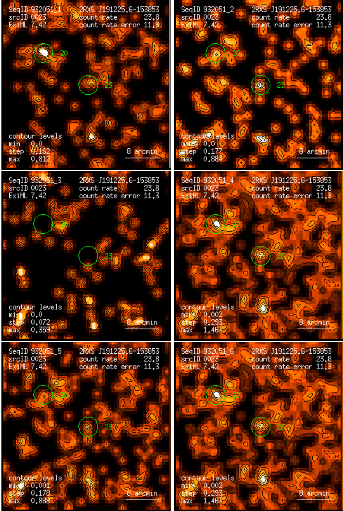
Figure 23: RASS 932051: detection 0023: band rate images, Gaussian filter: (1) PSPC channels 11 – 41, (2) 52 – 90, (3) 91 – 201, (4) 11 – 235, (5) 52 – 201, (6) 11 – 201. Broad band rates in counts/ks. Band rate contour levels in counts/ks/arcmin 2 .
