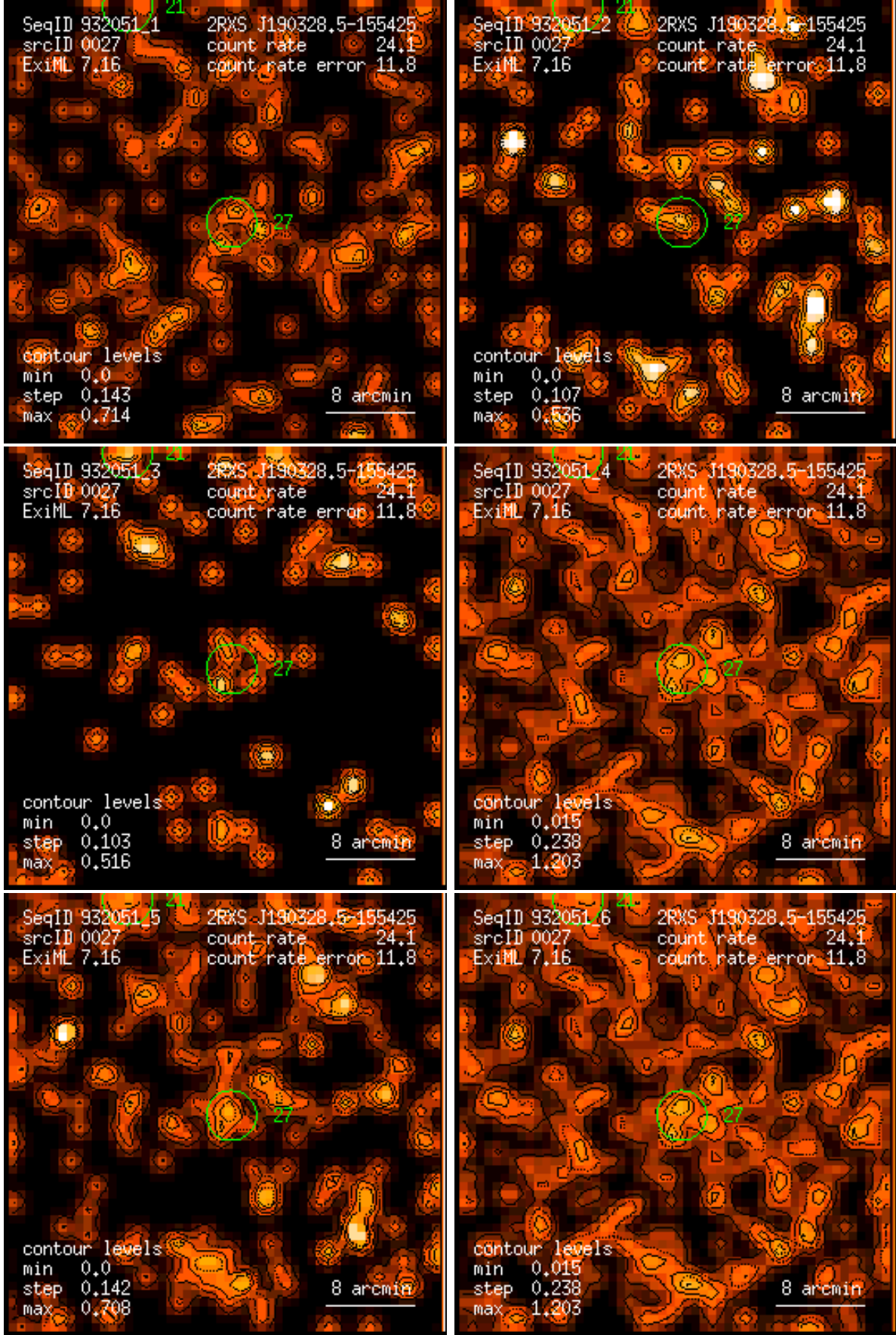
Figure 27: RASS 932051: detection 0027: band rate images, Gaussian filter: (1) PSPC channels 11 – 41, (2) 52 – 90, (3) 91 – 201, (4) 11 – 235, (5) 52 – 201, (6) 11 – 201. Broad band rates in counts/ks. Band rate contour levels in counts/ks/arcmin 2 .
