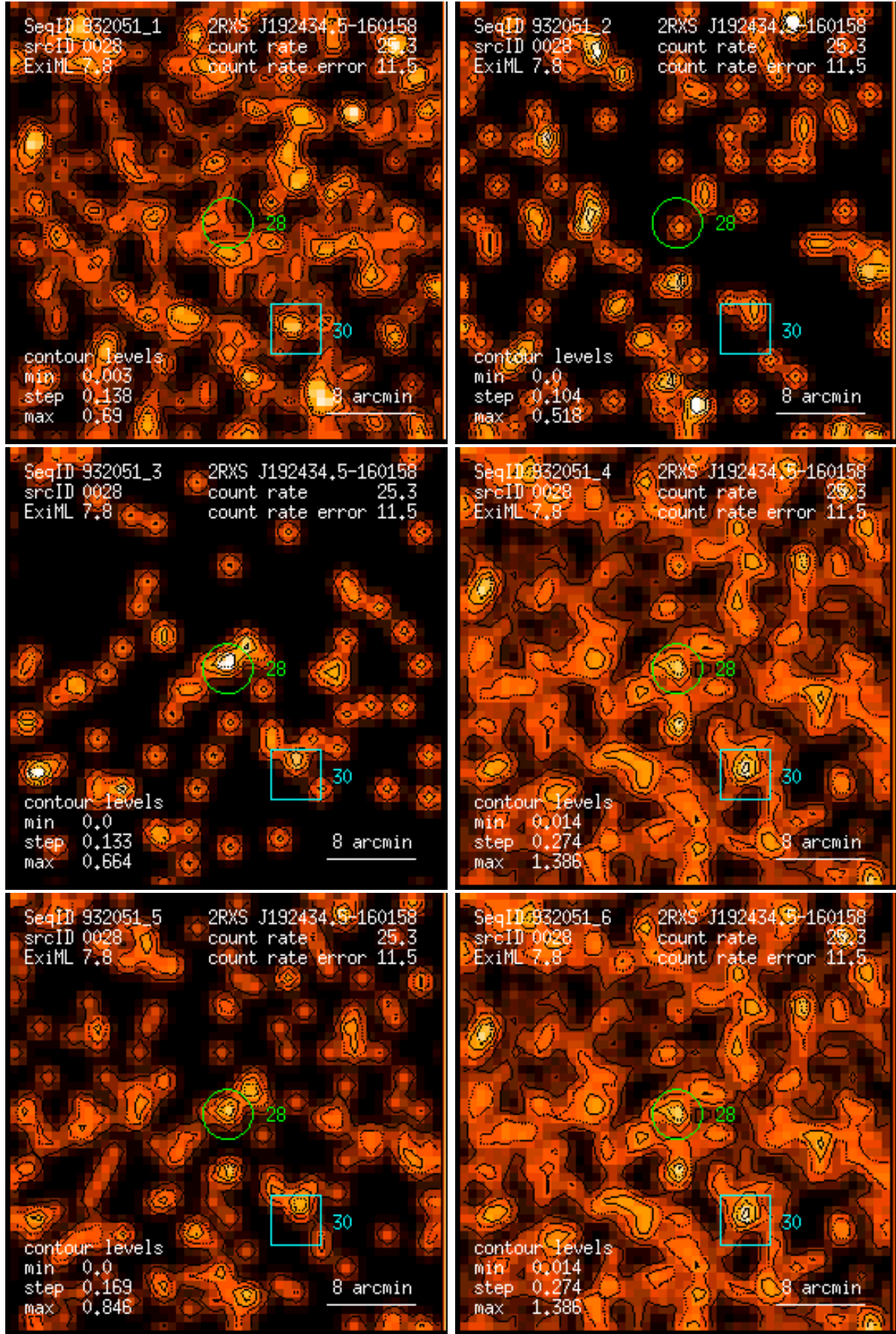
Figure 28: RASS 932051: detection 0028: band rate images, Gaussian filter: (1) PSPC channels 11 – 41, (2) 52 – 90, (3) 91 – 201, (4) 11 – 235, (5) 52 – 201, (6) 11 – 201. Broad band rates in counts/ks. Band rate contour levels in counts/ks/arcmin 2 .
