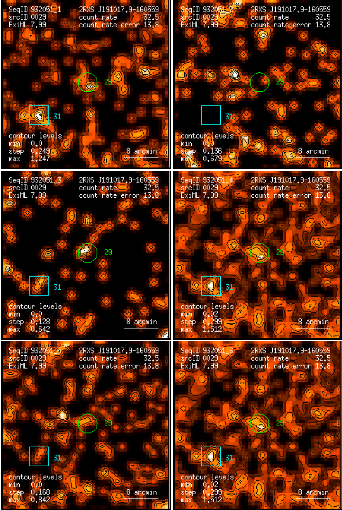
Figure 29: RASS 932051: detection 0029: band rate images, Gaussian filter: (1) PSPC channels 11 – 41, (2) 52 – 90, (3) 91 – 201, (4) 11 – 235, (5) 52 – 201, (6) 11 – 201. Broad band rates in counts/ks. Band rate contour levels in counts/ks/arcmin 2 .
