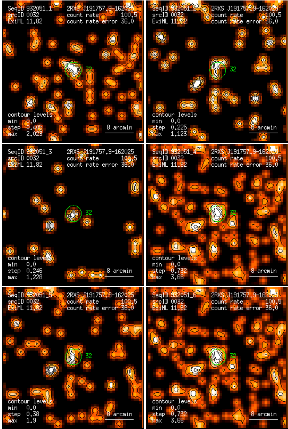
Figure 32: RASS 932051: detection 0032: band rate images, Gaussian filter: (1) PSPC channels 11 – 41, (2) 52 – 90, (3) 91 – 201, (4) 11 – 235, (5) 52 – 201, (6) 11 – 201. Broad band rates in counts/ks. Band rate contour levels in counts/ks/arcmin 2 .
