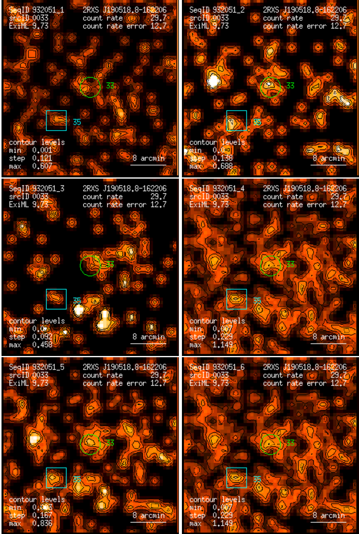
Figure 33: RASS 932051: detection 0033: band rate images, Gaussian filter: (1) PSPC channels 11 – 41, (2) 52 – 90, (3) 91 – 201, (4) 11 – 235, (5) 52 – 201, (6) 11 – 201. Broad band rates in counts/ks. Band rate contour levels in counts/ks/arcmin 2 .
