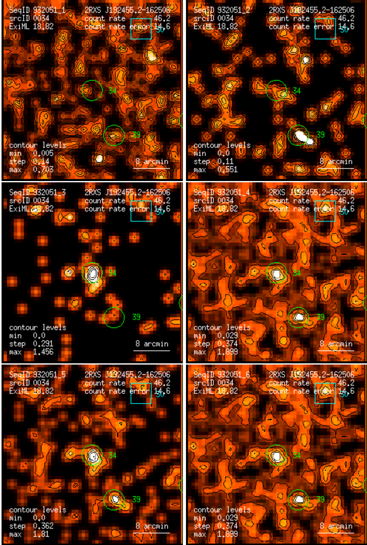
Figure 34: RASS 932051: detection 0034: band rate images, Gaussian filter: (1) PSPC channels 11 – 41, (2) 52 – 90, (3) 91 – 201, (4) 11 – 235, (5) 52 – 201, (6) 11 – 201. Broad band rates in counts/ks. Band rate contour levels in counts/ks/arcmin 2 .
