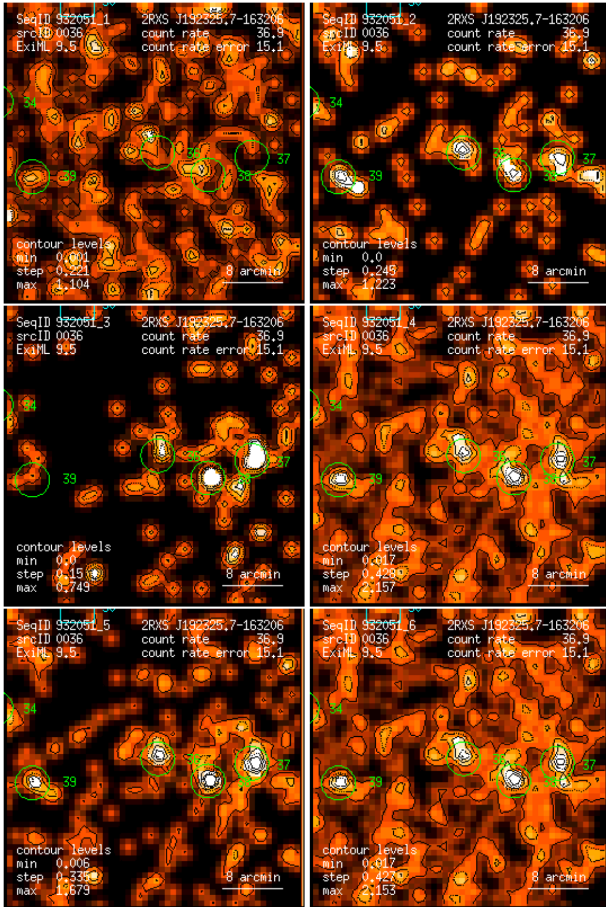
Figure 36: RASS 932051: detection 0036: band rate images, Gaussian filter: (1) PSPC channels 11 – 41, (2) 52 – 90, (3) 91 – 201, (4) 11 – 235, (5) 52 – 201, (6) 11 – 201. Broad band rates in counts/ks. Band rate contour levels in counts/ks/arcmin 2 .
