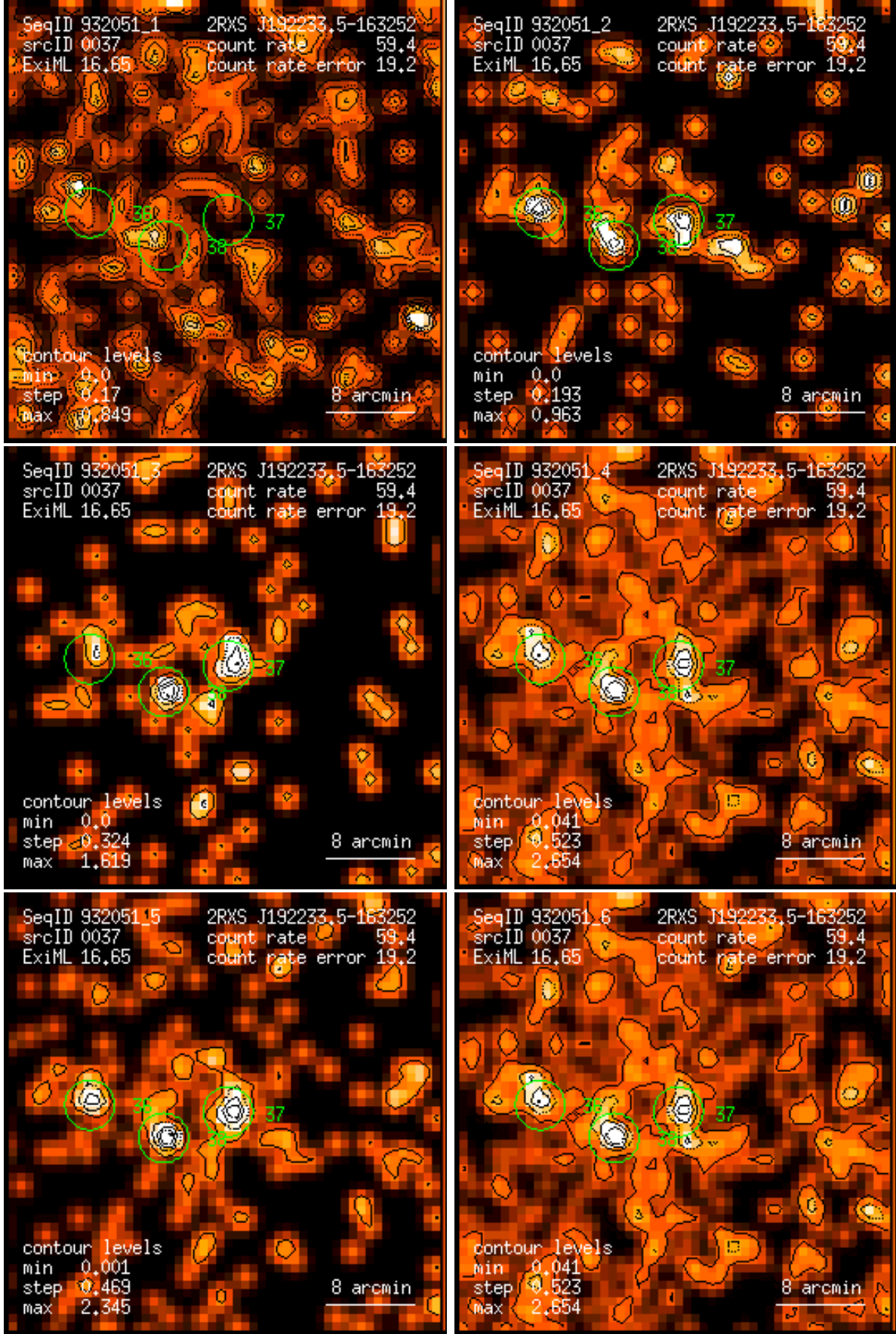
Figure 37: RASS 932051: detection 0037: band rate images, Gaussian filter: (1) PSPC channels 11 – 41, (2) 52 – 90, (3) 91 – 201, (4) 11 – 235, (5) 52 – 201, (6) 11 – 201. Broad band rates in counts/ks. Band rate contour levels in counts/ks/arcmin 2 .
