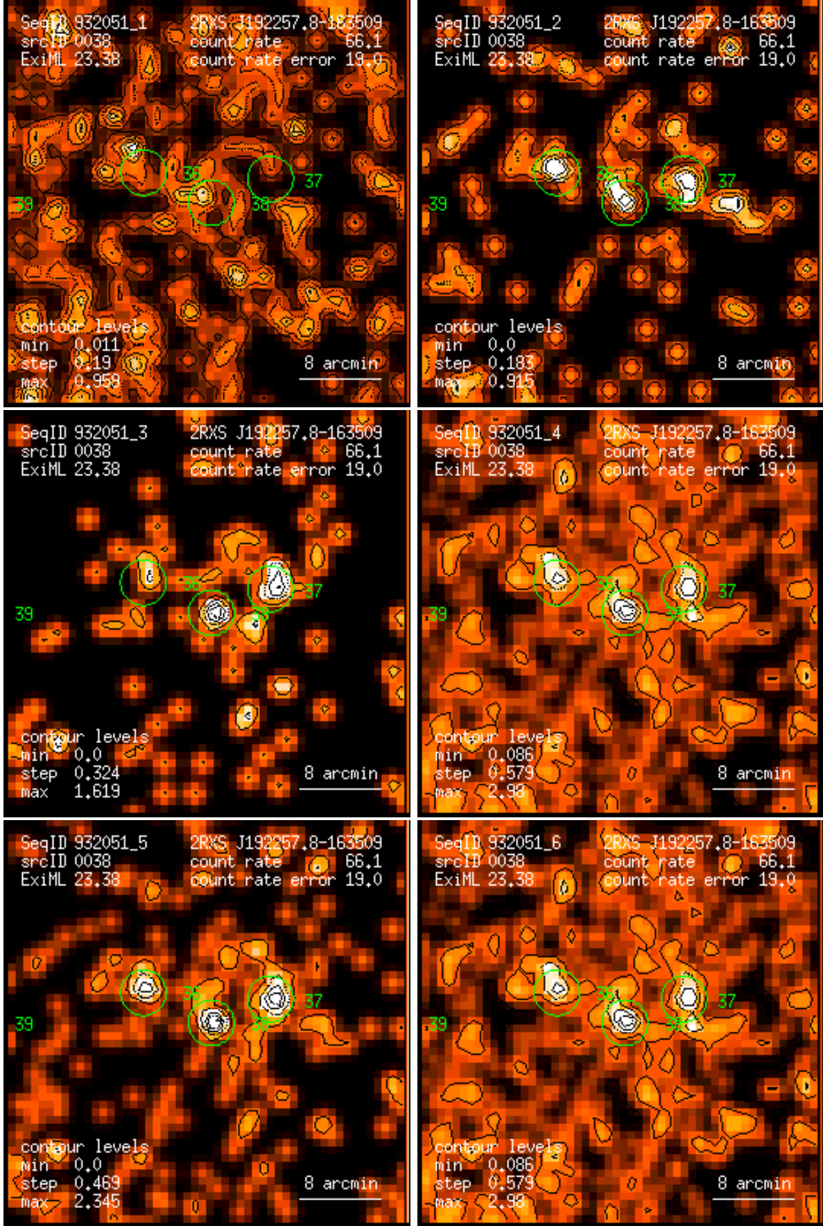
Figure 38: RASS 932051: detection 0038: band rate images, Gaussian filter: (1) PSPC channels 11 – 41, (2) 52 – 90, (3) 91 – 201, (4) 11 – 235, (5) 52 – 201, (6) 11 – 201. Broad band rates in counts/ks. Band rate contour levels in counts/ks/arcmin 2 .
