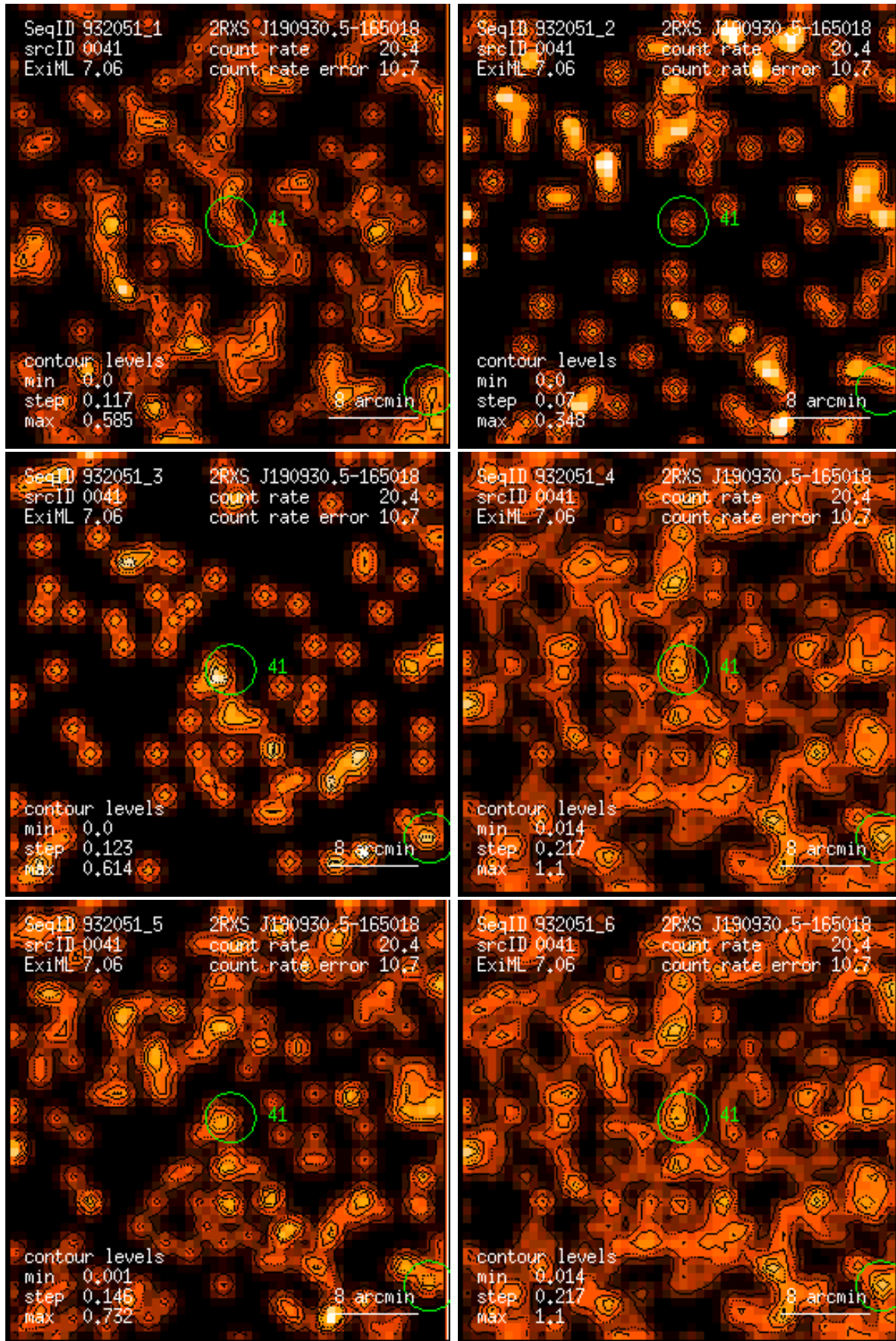
Figure 41: RASS 932051: detection 0041: band rate images, Gaussian filter: (1) PSPC channels 11 – 41, (2) 52 – 90, (3) 91 – 201, (4) 11 – 235, (5) 52 – 201, (6) 11 – 201. Broad band rates in counts/ks. Band rate contour levels in counts/ks/arcmin 2 .
