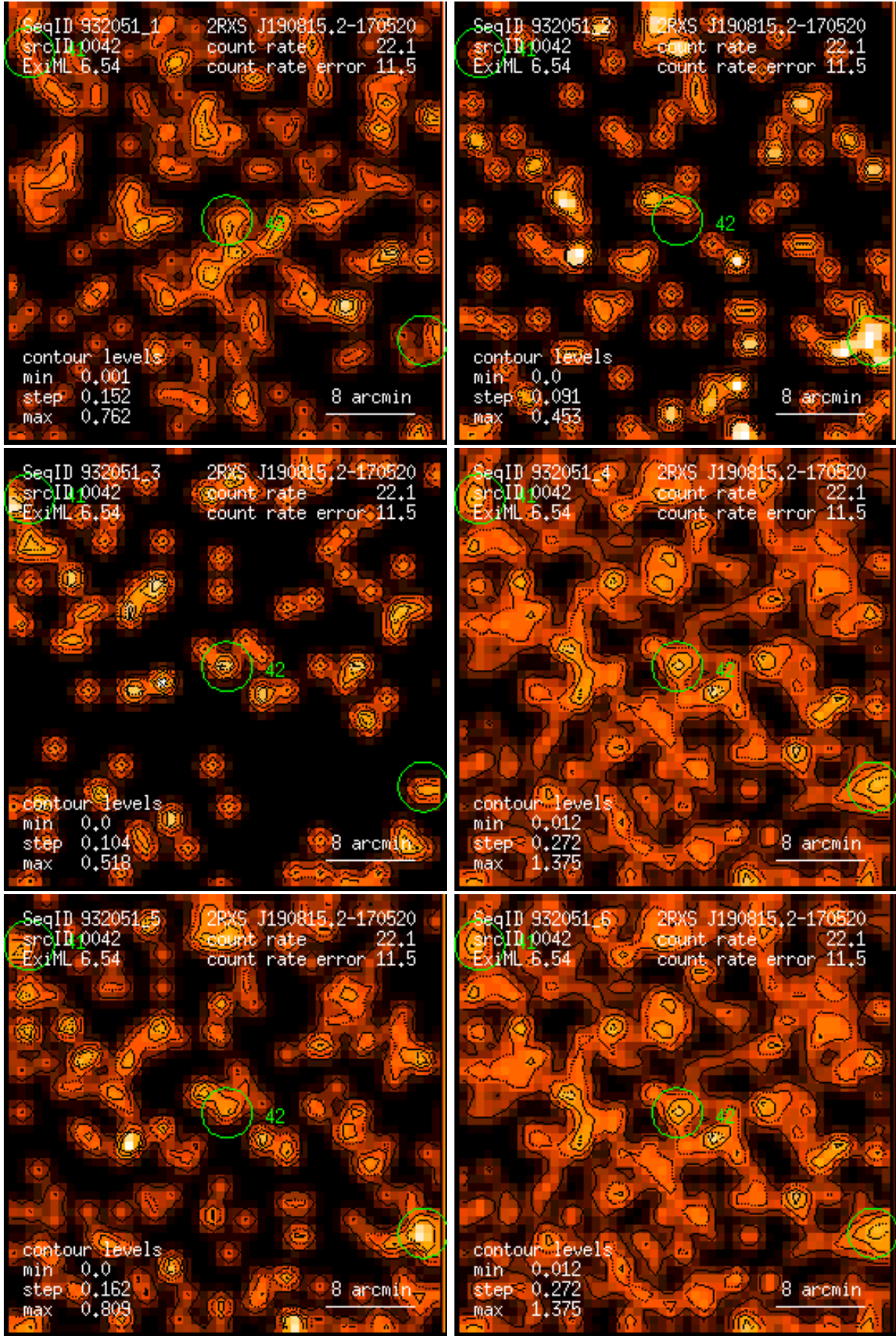
Figure 42: RASS 932051: detection 0042: band rate images, Gaussian filter: (1) PSPC channels 11 – 41, (2) 52 – 90, (3) 91 – 201, (4) 11 – 235, (5) 52 – 201, (6) 11 – 201. Broad band rates in counts/ks. Band rate contour levels in counts/ks/arcmin 2 .
