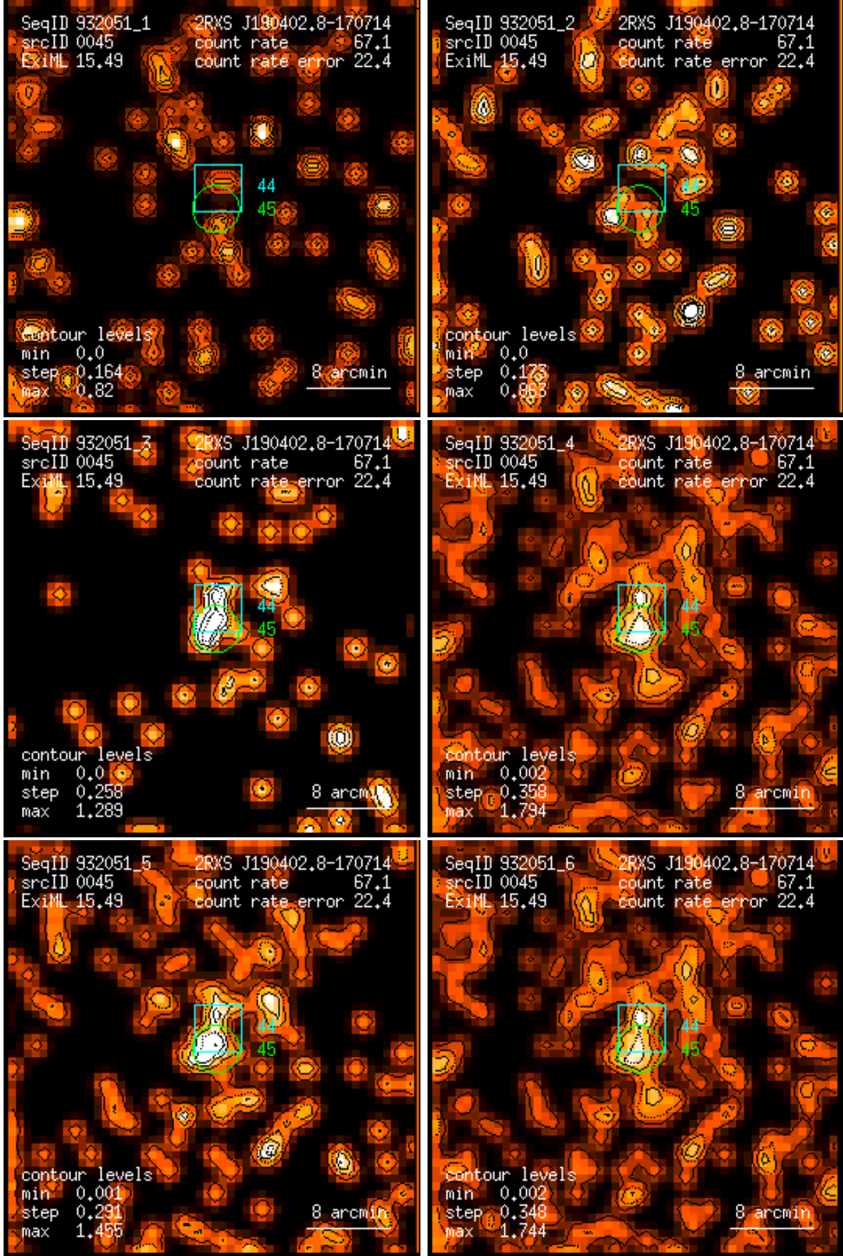
Figure 45: RASS 932051: detection 0045: band rate images, Gaussian filter: (1) PSPC channels 11 – 41, (2) 52 – 90, (3) 91 – 201, (4) 11 – 235, (5) 52 – 201, (6) 11 – 201. Broad band rates in counts/ks. Band rate contour levels in counts/ks/arcmin 2 .
