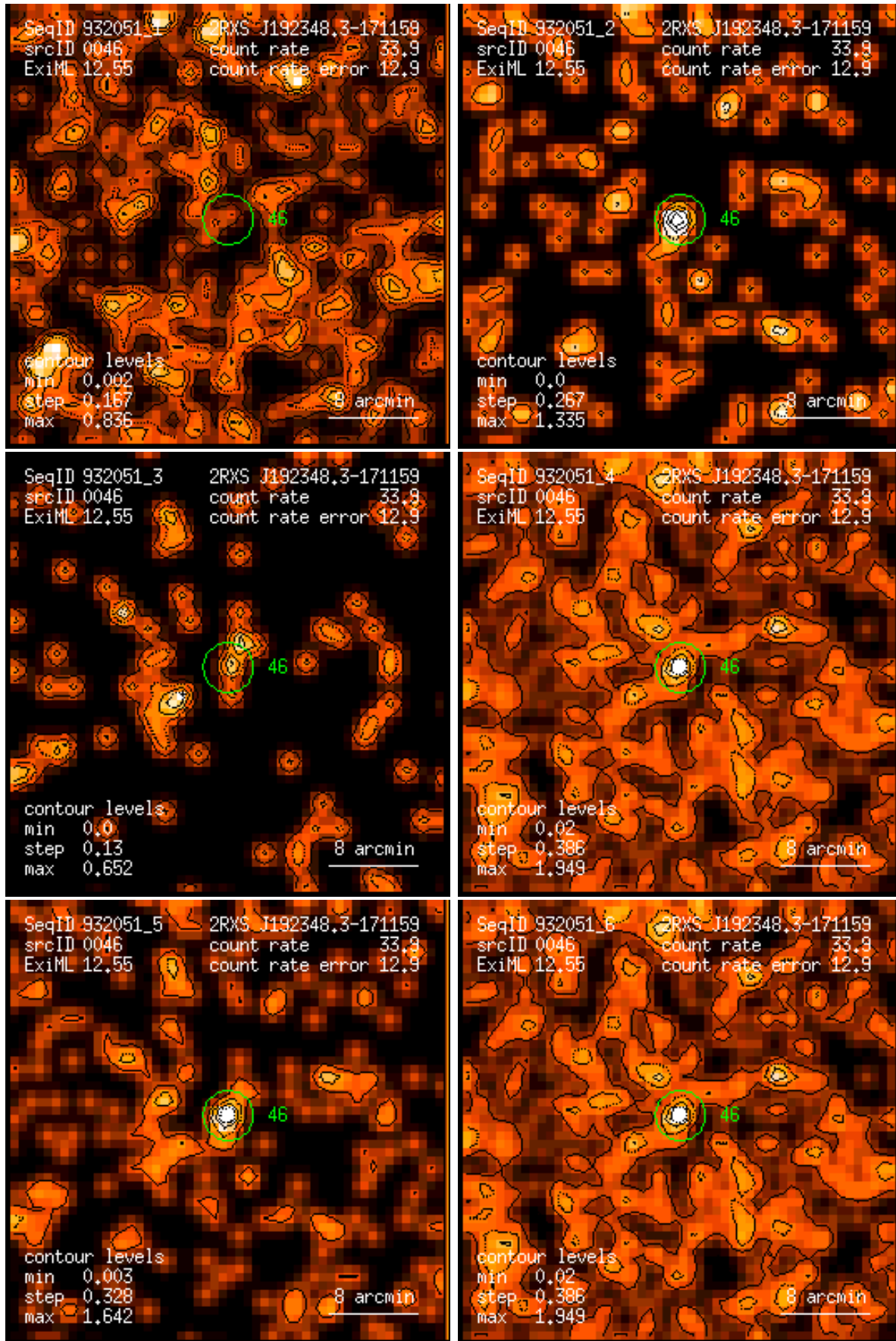
Figure 46: RASS 932051: detection 0046: band rate images, Gaussian filter: (1) PSPC channels 11 – 41, (2) 52 – 90, (3) 91 – 201, (4) 11 – 235, (5) 52 – 201, (6) 11 – 201. Broad band rates in counts/ks. Band rate contour levels in counts/ks/arcmin 2 .
