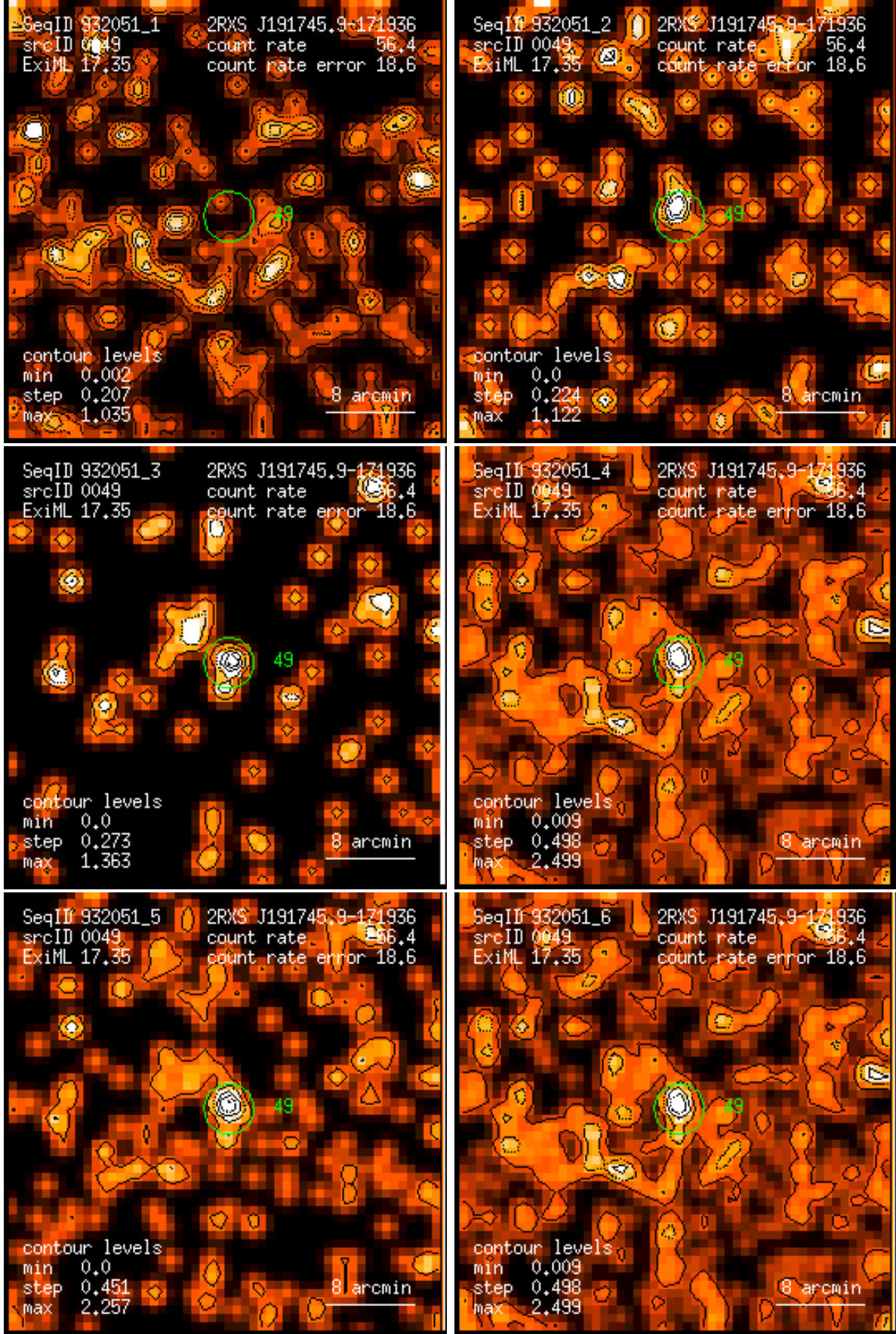
Figure 49: RASS 932051: detection 0049: band rate images, Gaussian filter: (1) PSPC channels 11 – 41, (2) 52 – 90, (3) 91 – 201, (4) 11 – 235, (5) 52 – 201, (6) 11 – 201. Broad band rates in counts/ks. Band rate contour levels in counts/ks/arcmin 2 .
