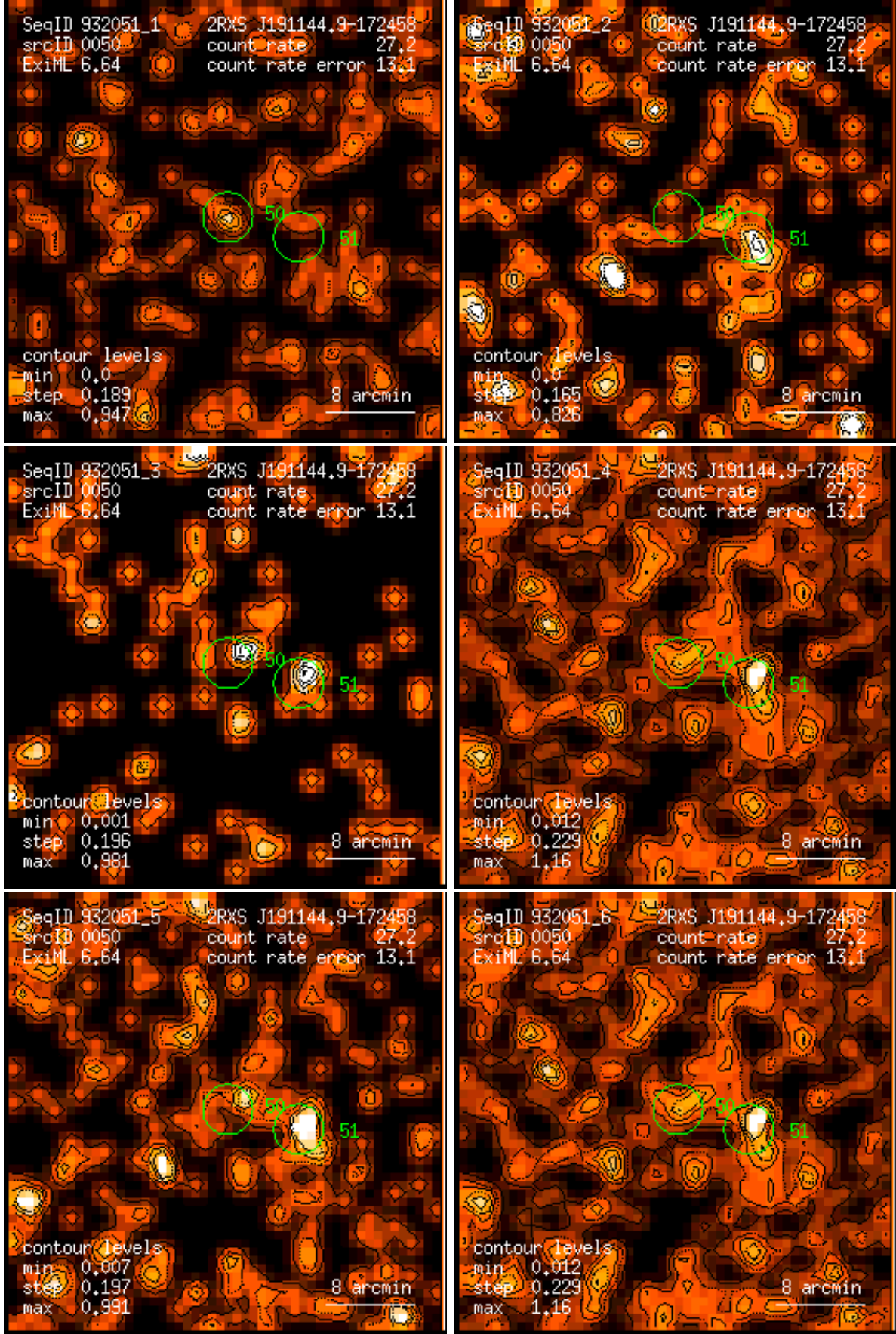
Figure 50: RASS 932051: detection 0050: band rate images, Gaussian filter: (1) PSPC channels 11 – 41, (2) 52 – 90, (3) 91 – 201, (4) 11 – 235, (5) 52 – 201, (6) 11 – 201. Broad band rates in counts/ks. Band rate contour levels in counts/ks/arcmin 2 .
