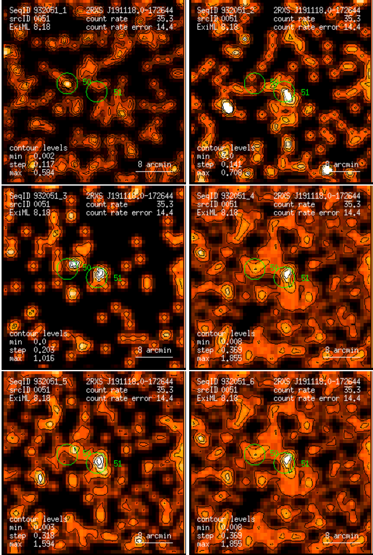
Figure 51: RASS 932051: detection 0051: band rate images, Gaussian filter: (1) PSPC channels 11 – 41, (2) 52 – 90, (3) 91 – 201, (4) 11 – 235, (5) 52 – 201, (6) 11 – 201. Broad band rates in counts/ks. Band rate contour levels in counts/ks/arcmin 2 .
