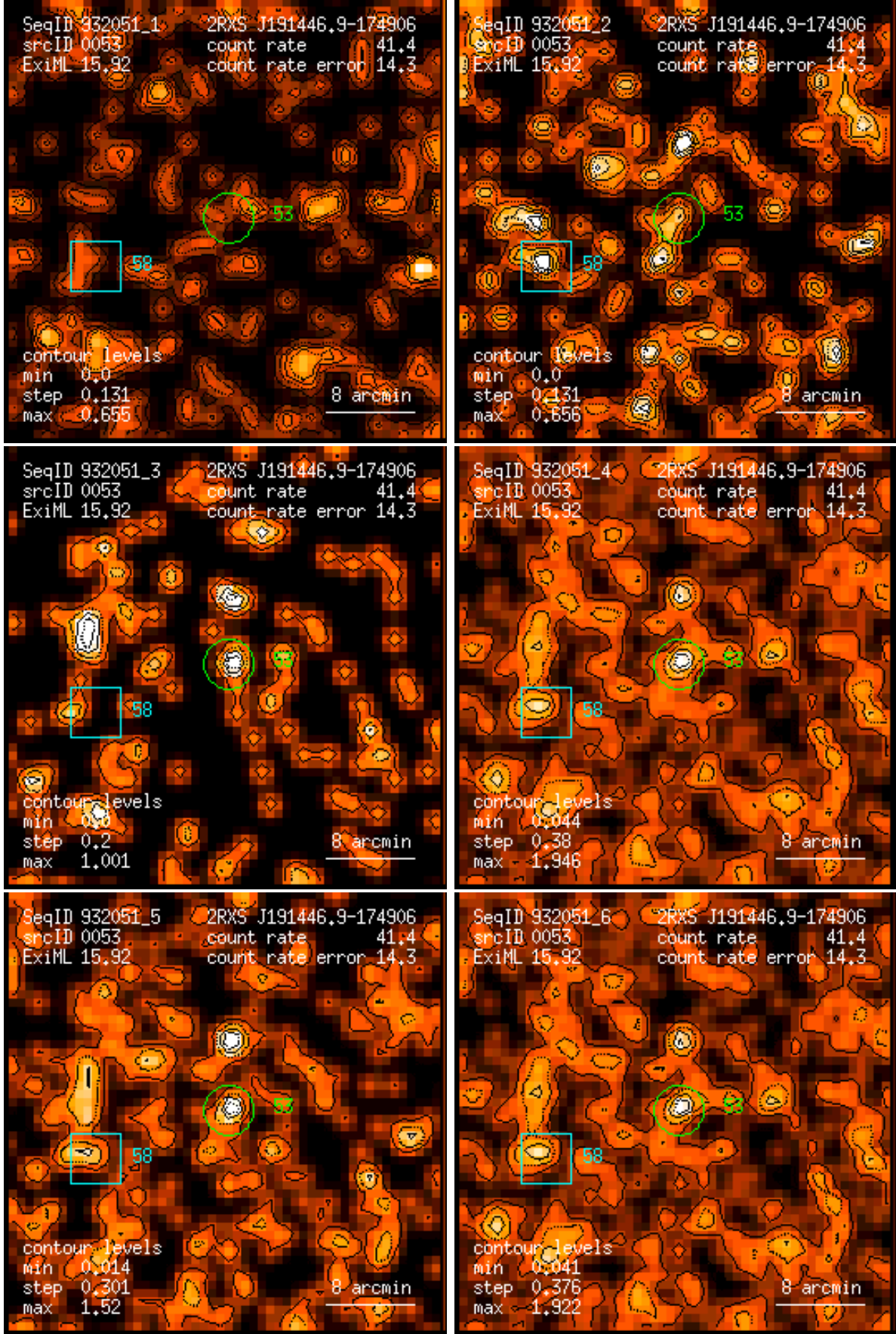
Figure 53: RASS 932051: detection 0053: band rate images, Gaussian filter: (1) PSPC channels 11 – 41, (2) 52 – 90, (3) 91 – 201, (4) 11 – 235, (5) 52 – 201, (6) 11 – 201. Broad band rates in counts/ks. Band rate contour levels in counts/ks/arcmin 2 .
