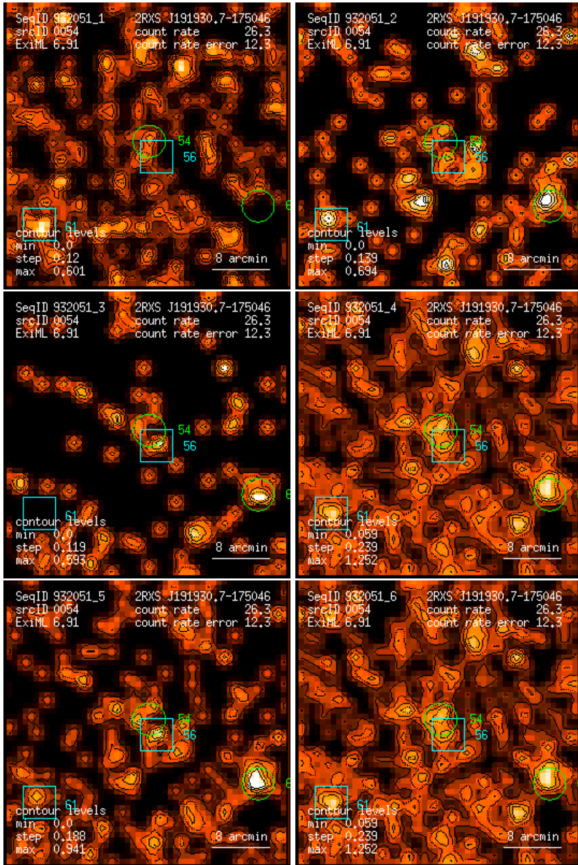
Figure 54: RASS 932051: detection 0054: band rate images, Gaussian filter: (1) PSPC channels 11 – 41, (2) 52 – 90, (3) 91 – 201, (4) 11 – 235, (5) 52 – 201, (6) 11 – 201. Broad band rates in counts/ks. Band rate contour levels in counts/ks/arcmin 2 .
