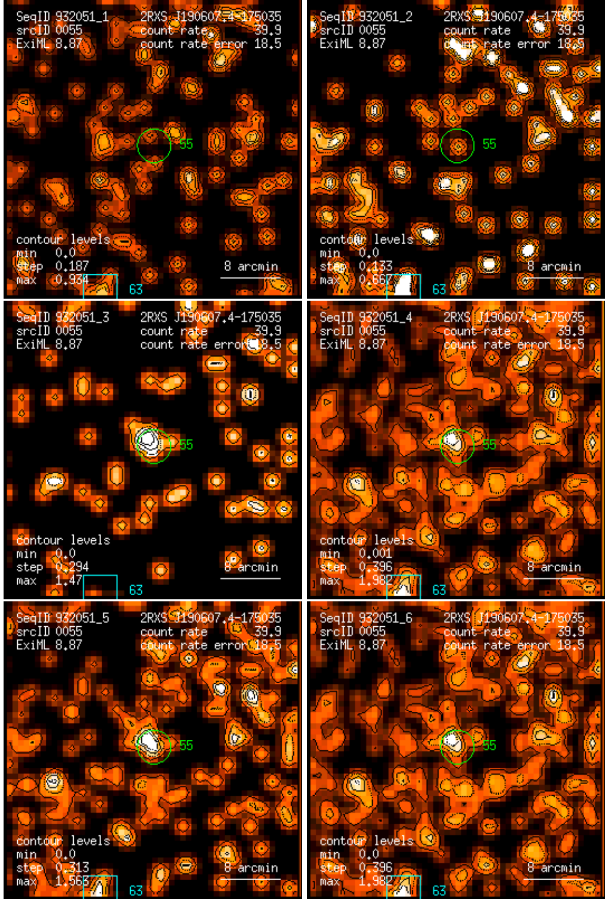
Figure 55: RASS 932051: detection 0055: band rate images, Gaussian filter: (1) PSPC channels 11 – 41, (2) 52 – 90, (3) 91 – 201, (4) 11 – 235, (5) 52 – 201, (6) 11 – 201. Broad band rates in counts/ks. Band rate contour levels in counts/ks/arcmin 2 .
