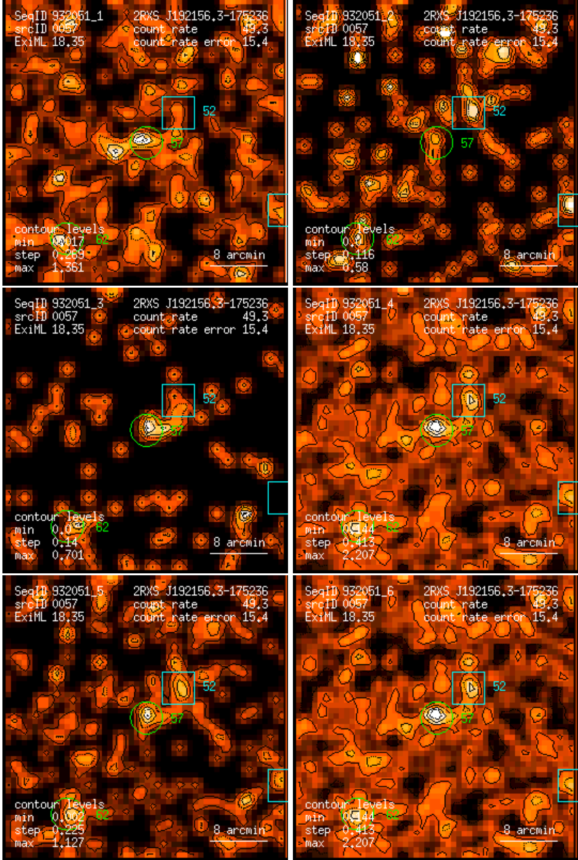
Figure 57: RASS 932051: detection 0057: band rate images, Gaussian filter: (1) PSPC channels 11 – 41, (2) 52 – 90, (3) 91 – 201, (4) 11 – 235, (5) 52 – 201, (6) 11 – 201. Broad band rates in counts/ks. Band rate contour levels in counts/ks/arcmin 2 .
