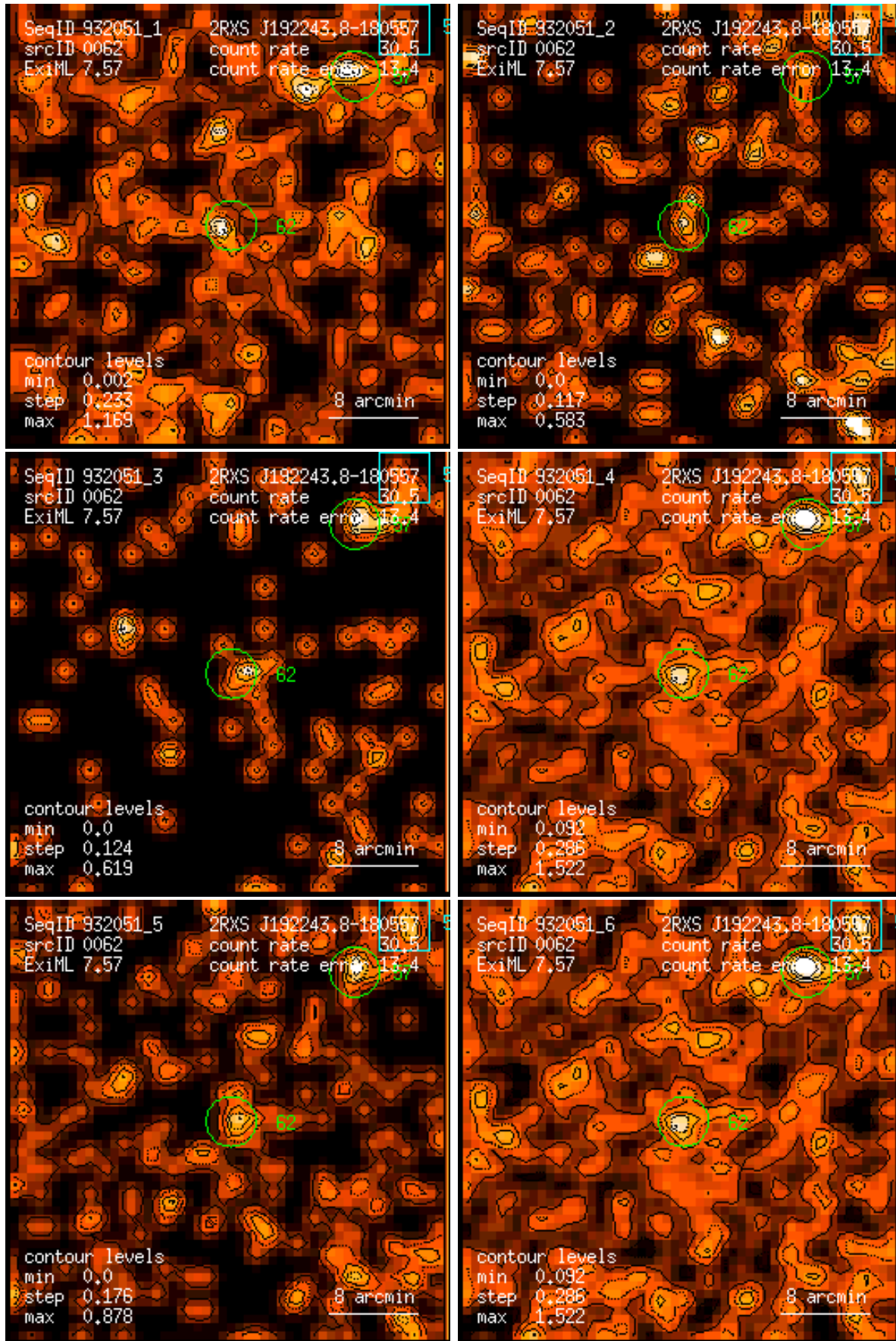
Figure 62: RASS 932051: detection 0062: band rate images, Gaussian filter: (1) PSPC channels 11 – 41, (2) 52 – 90, (3) 91 – 201, (4) 11 – 235, (5) 52 – 201, (6) 11 – 201. Broad band rates in counts/ks. Band rate contour levels in counts/ks/arcmin 2 .
