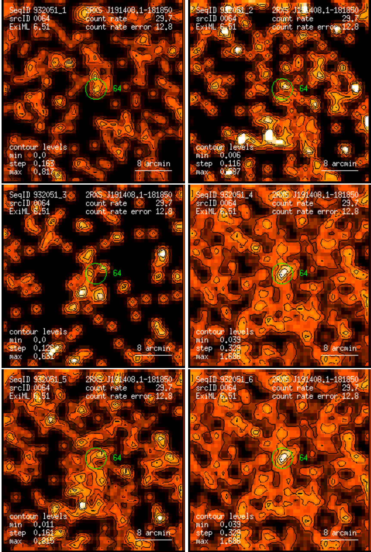
Figure 64: RASS 932051: detection 0064: band rate images, Gaussian filter: (1) PSPC channels 11 – 41, (2) 52 – 90, (3) 91 – 201, (4) 11 – 235, (5) 52 – 201, (6) 11 – 201. Broad band rates in counts/ks. Band rate contour levels in counts/ks/arcmin 2 .
