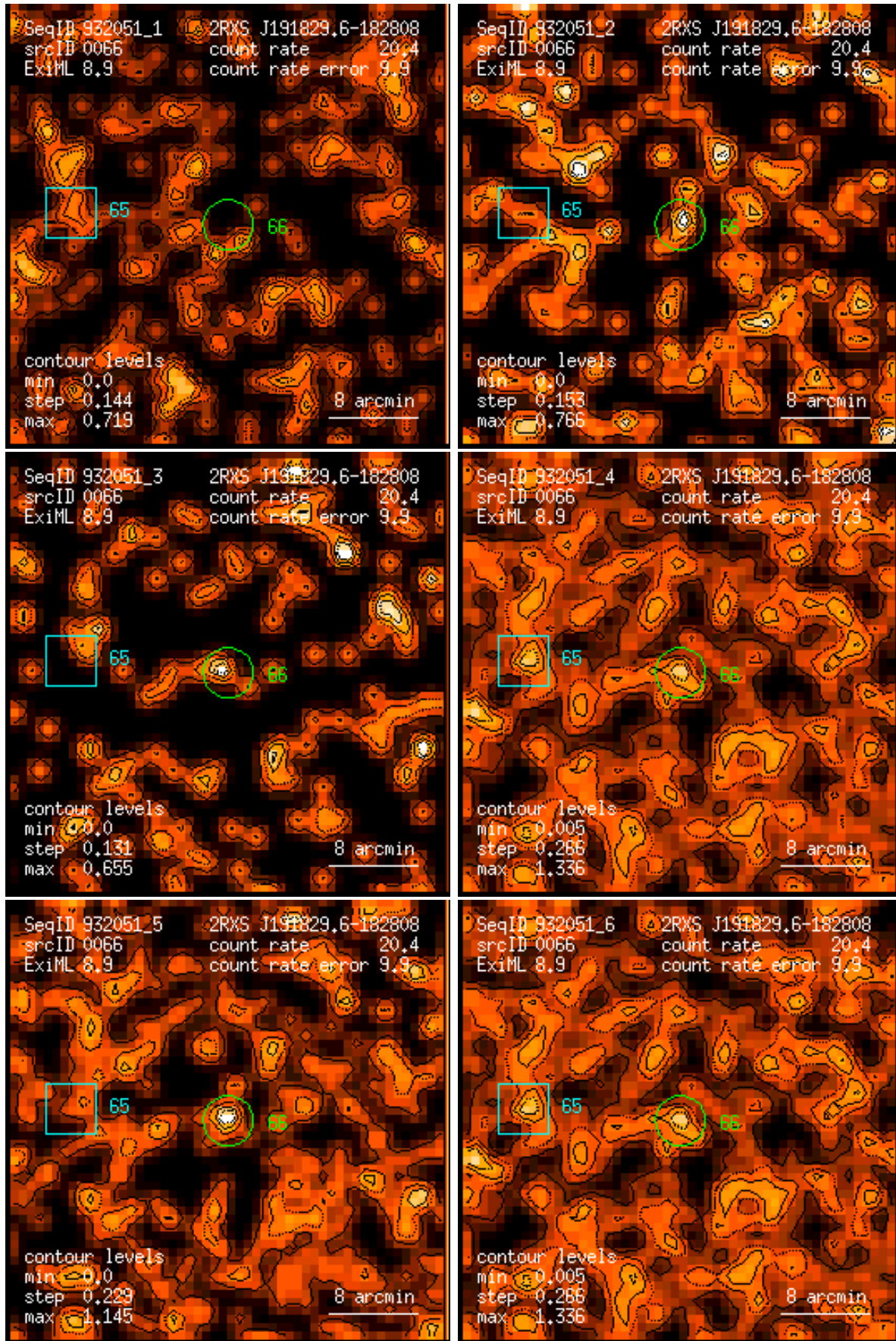
Figure 66: RASS 932051: detection 0066: band rate images, Gaussian filter: (1) PSPC channels 11 – 41, (2) 52 – 90, (3) 91 – 201, (4) 11 – 235, (5) 52 – 201, (6) 11 – 201. Broad band rates in counts/ks. Band rate contour levels in counts/ks/arcmin 2 .
