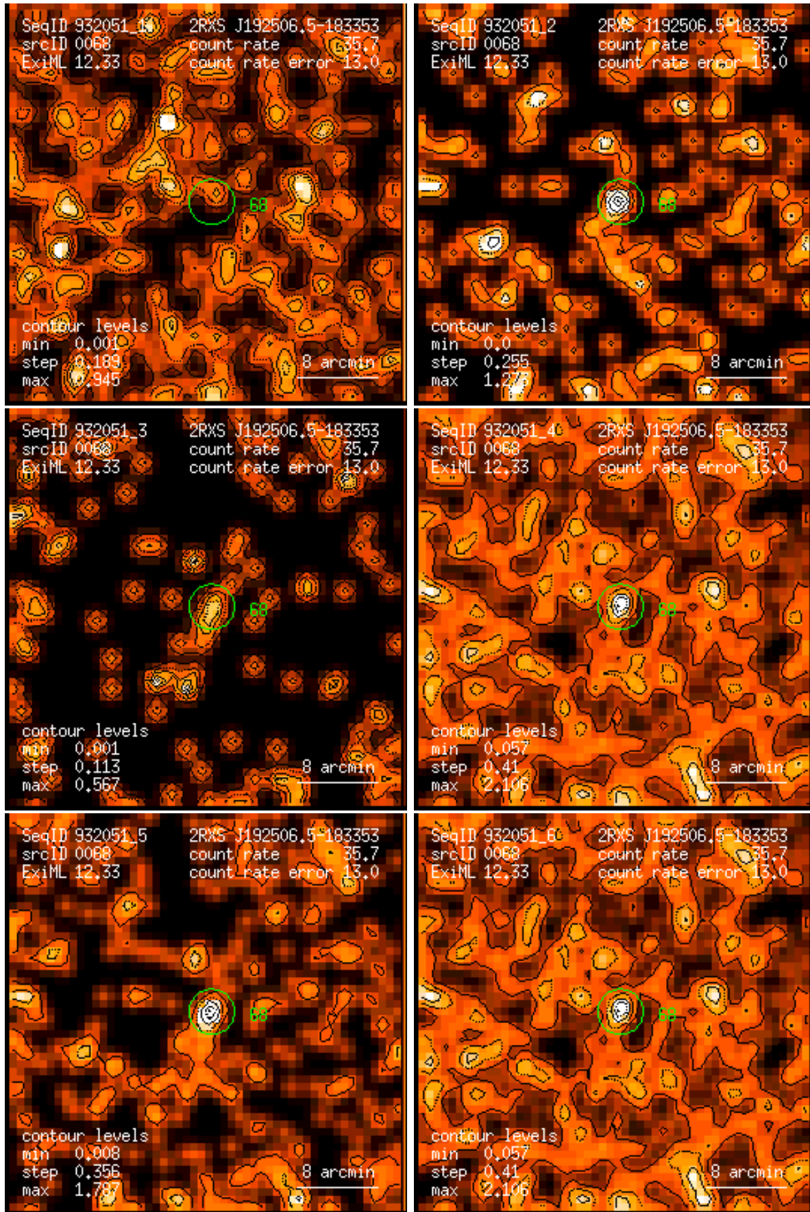
Figure 68: RASS 932051: detection 0068: band rate images, Gaussian filter: (1) PSPC channels 11 – 41, (2) 52 – 90, (3) 91 – 201, (4) 11 – 235, (5) 52 – 201, (6) 11 – 201. Broad band rates in counts/ks. Band rate contour levels in counts/ks/arcmin 2 .
