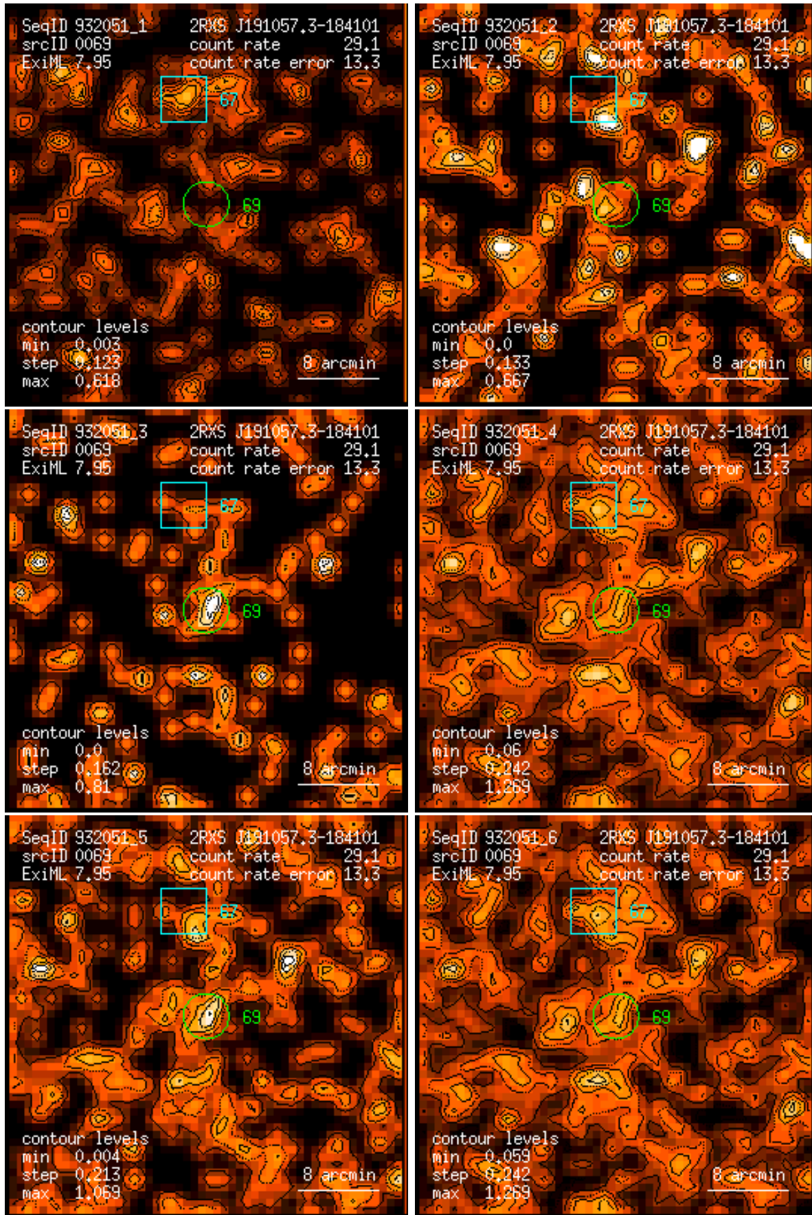
Figure 69: RASS 932051: detection 0069: band rate images, Gaussian filter: (1) PSPC channels 11 – 41, (2) 52 – 90, (3) 91 – 201, (4) 11 – 235, (5) 52 – 201, (6) 11 – 201. Broad band rates in counts/ks. Band rate contour levels in counts/ks/arcmin 2 .
